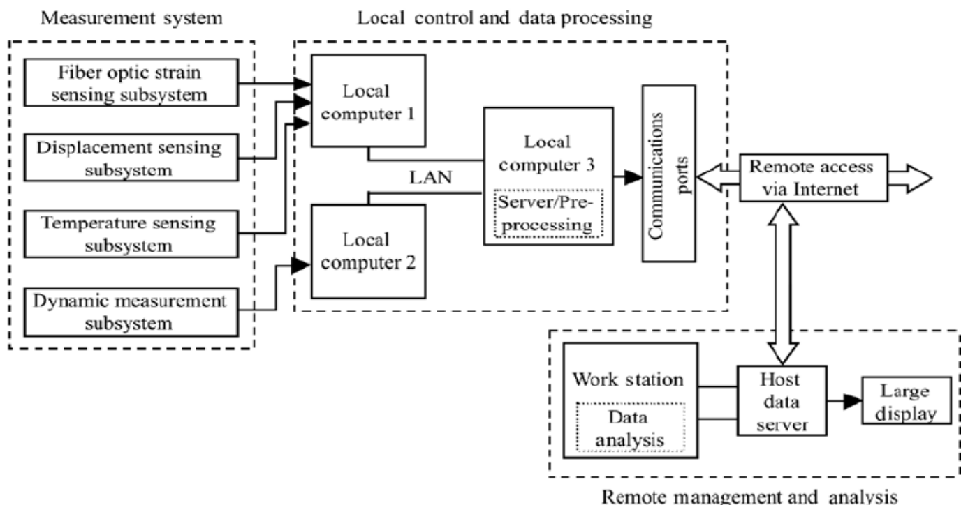
Figure 3. Schematic Diagram of Bridge Health Monitoring System
