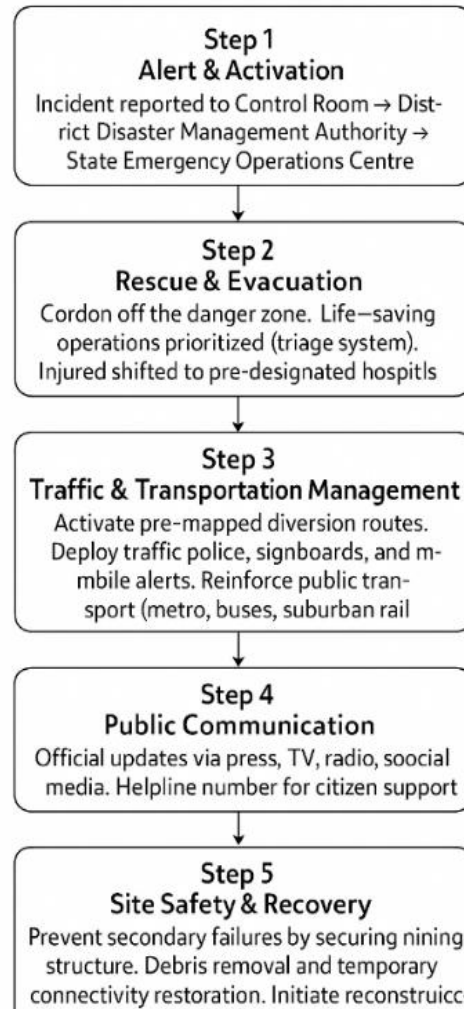
Fig 2. SOP Flowchart: Bridge Collapse Disaster Management
