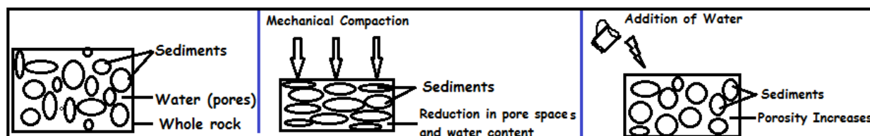
Fig. 2: Image of rock constituents describing what happens during water saturation, compaction, and lithification.
