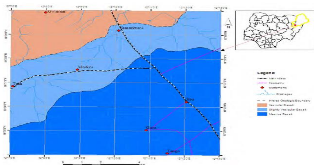
Fig. 1: Location geologic map of the study area
