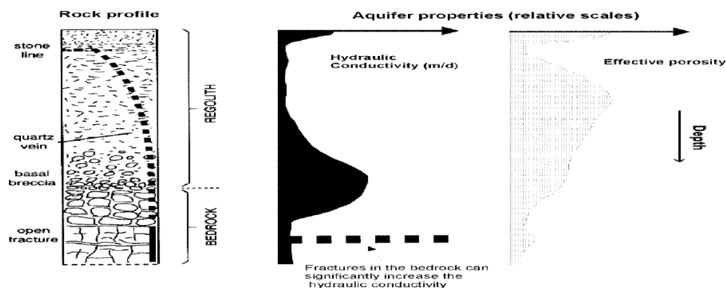
Figure 3: Variation of permeability and porosity with depth in basement aquifers (After Chilton and Foster, 1995)
