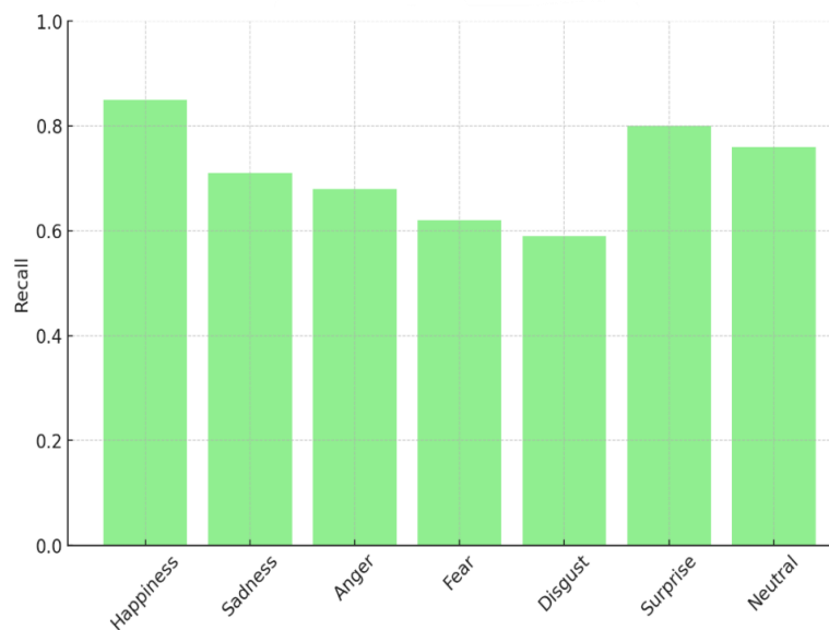
Fig. 3. Recall Scores for Emotion Recognition Across FER-2013 Dataset
