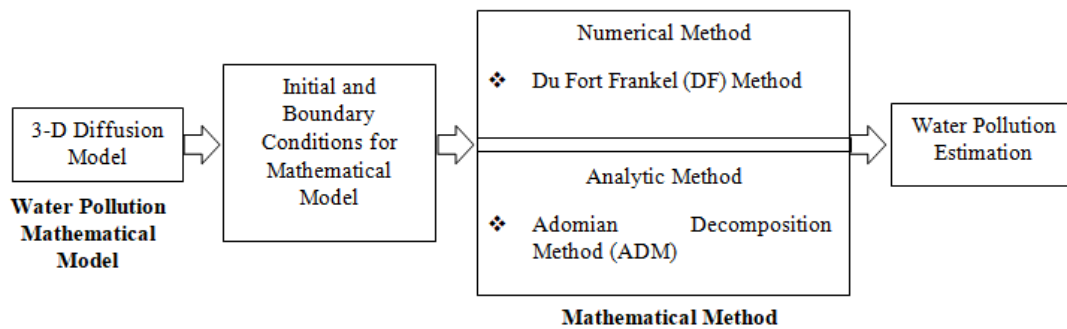
Fig. 1 Mathematical method for 3-D water pollution estimation
