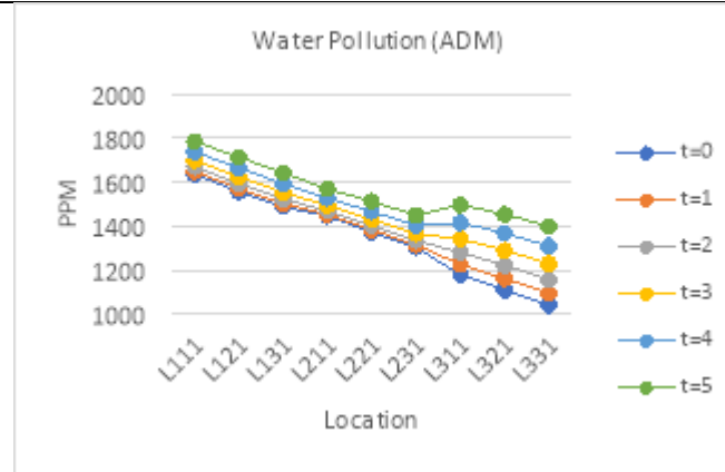
Fig. 10 DF, Exp. data and ADM Result at Nine Unknown Locations
