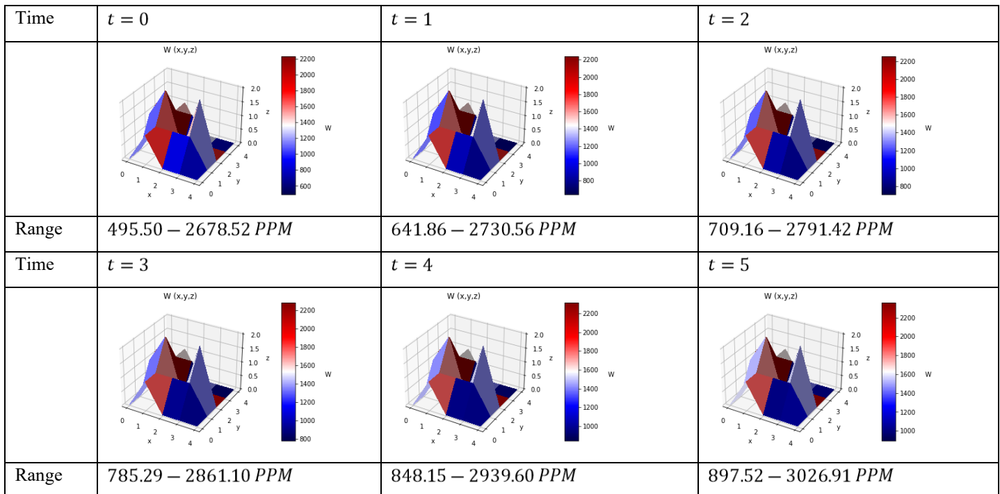
Fig. 7 Water pollution at 3-D grid locations by ADM
