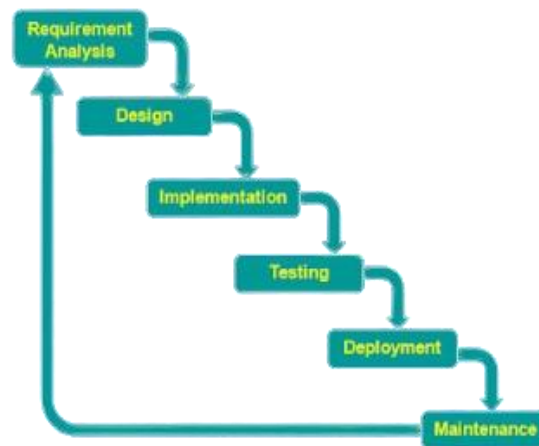
Figure 2: SDLC Model
