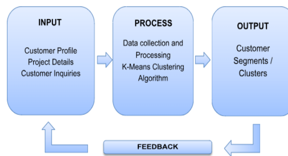
Figure 1: Input-Process-Output Mode
