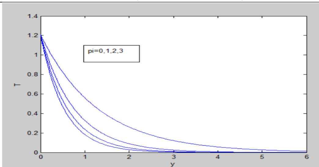
Fig3: Temperature T versus y under the effect of \pi(\phi)
