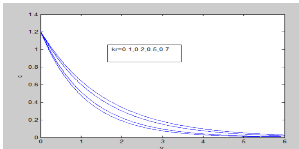
Fig2: Concentration versus y under the effects of Kr.
