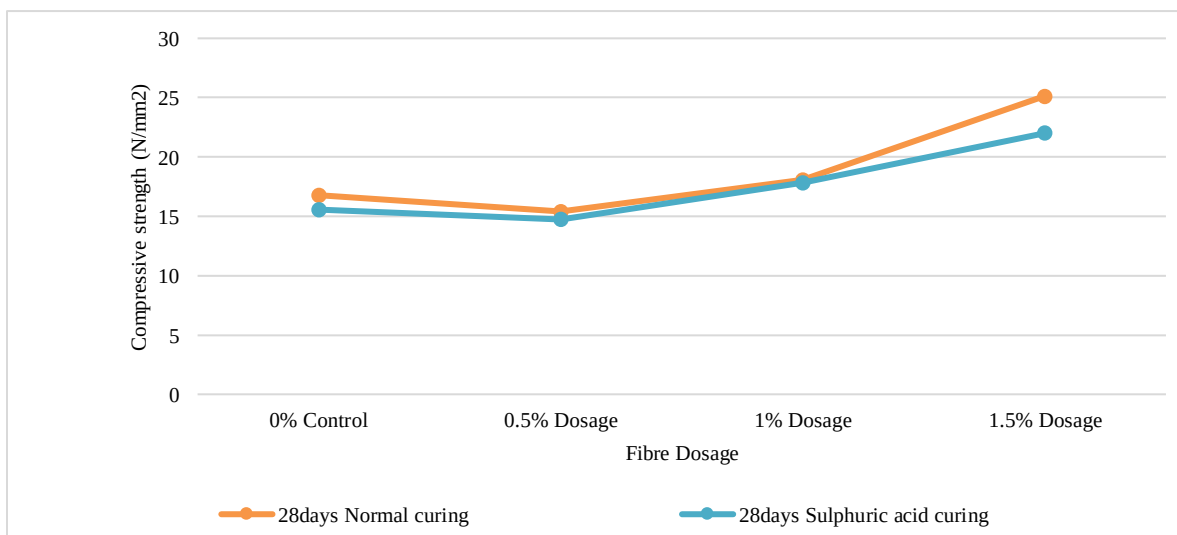
Figure 3: Effect of H_2SO_4 curing on Compressive strength of Concrete with PWTW after 28days
