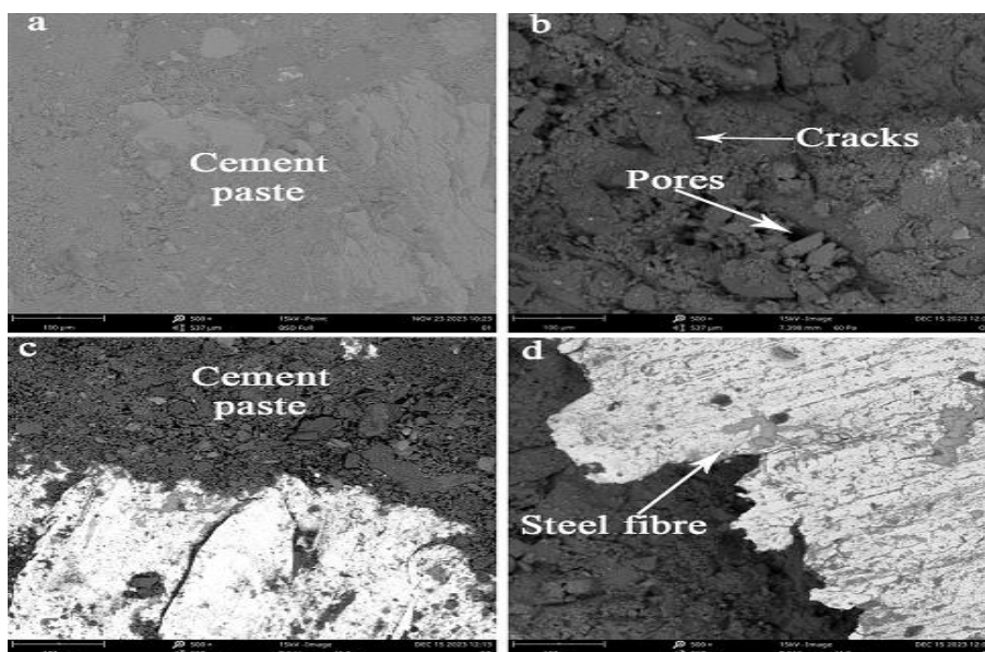
Figure 8: SEM Images of Concrete Samples before and after exposure to MgSO_4 , a) Control Sample Before; (b) Control Sample after; (c) 1.5% PWTW Concrete before exposure; (d) 1.5% PWTW Concrete after exposure
