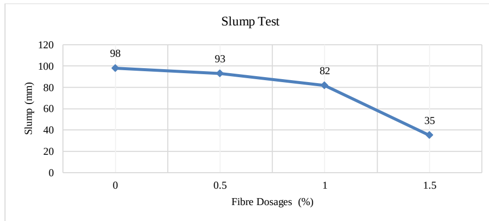
Figure 2: Slump Values at Fresh stage
