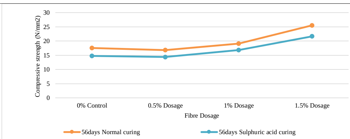
Figure 4: Effect of H_2SO_4 curing on Compressive strength of Concrete with PWTW after 56days
