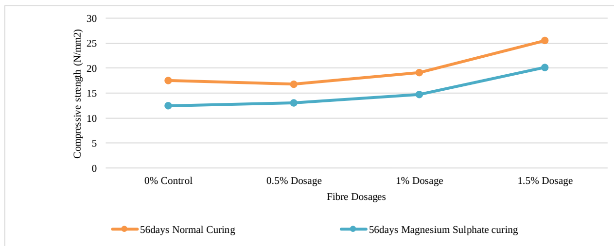
Figure 6: Effect of MgSO_4 curing on Compressive strength of Concrete with PWTW after 56days
