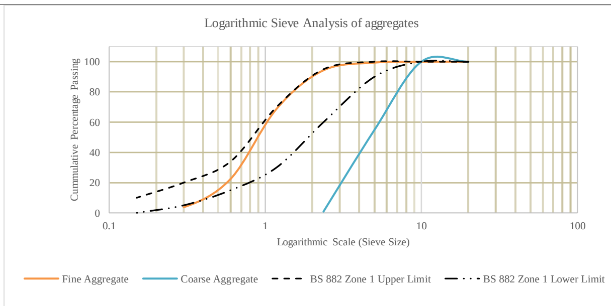
Figure 1: Particle Size Distribution of Aggregates
