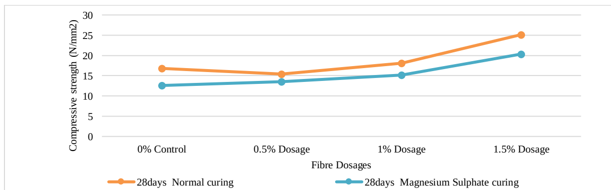
Figure 5: Effect of MgSO_4 curing on Compressive strength of Concrete with PWTW after 28days
