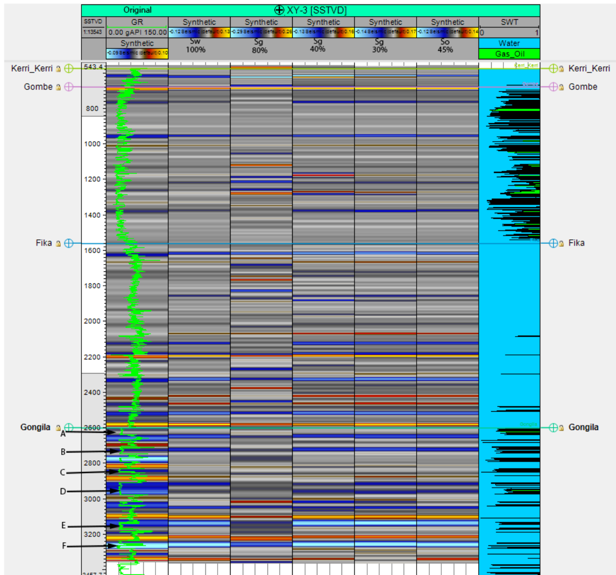
Figure 17: Seismic traces along well XY-3 for the original or in-situ measured data and those of the fluid substituted response for each of the scenario chosen to be tested.
