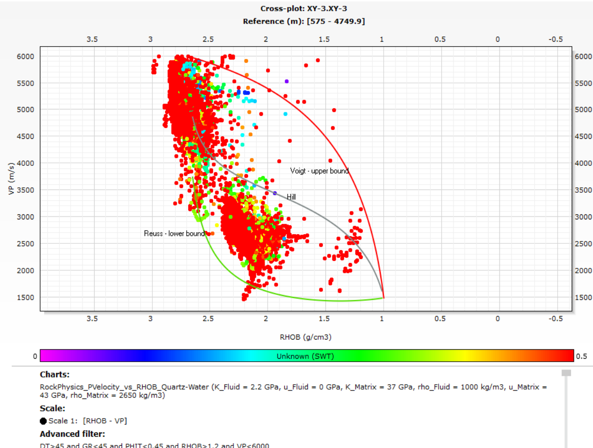
Figure 16: VP vs RhoB plot with the Voight-Hill-Reuss bound with filters applied to remove some of the effects of the background.
