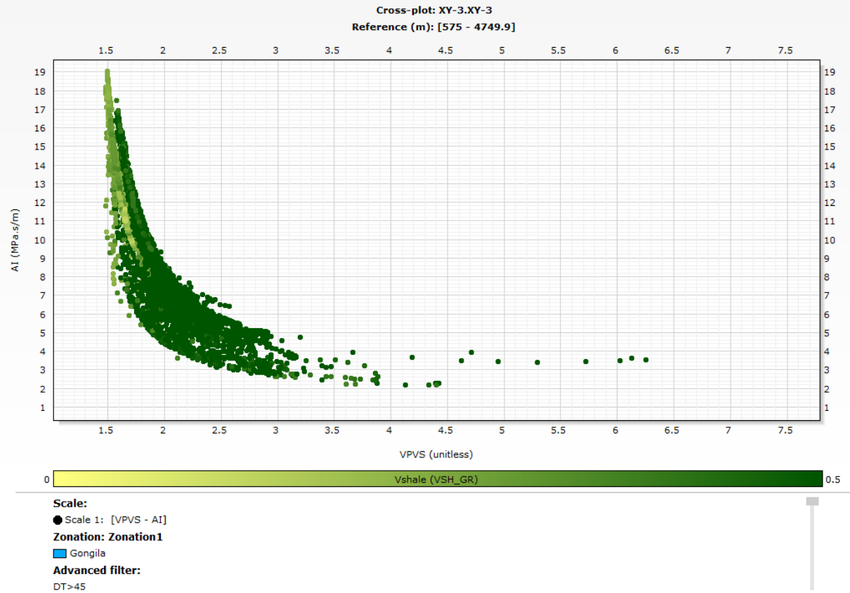
Figure 6: AI vs VPVS plot with background removed. The plot represents the measurements or responses from only the Gongila Formation reservoir interval.
