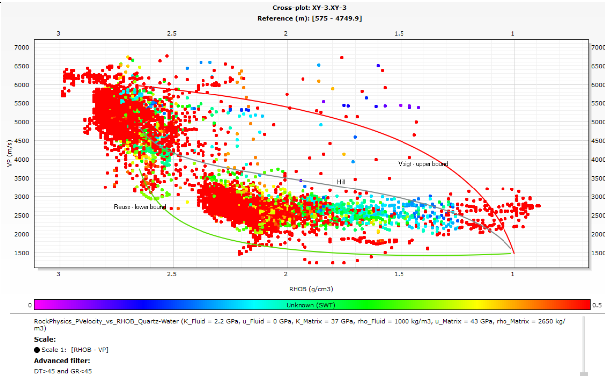
Figure 15: VP vs RhoB plot coloured by water saturation with the Voight-Hill-Reuss bound. The large variance or variability observed in the plot is due to the effect of the background.
