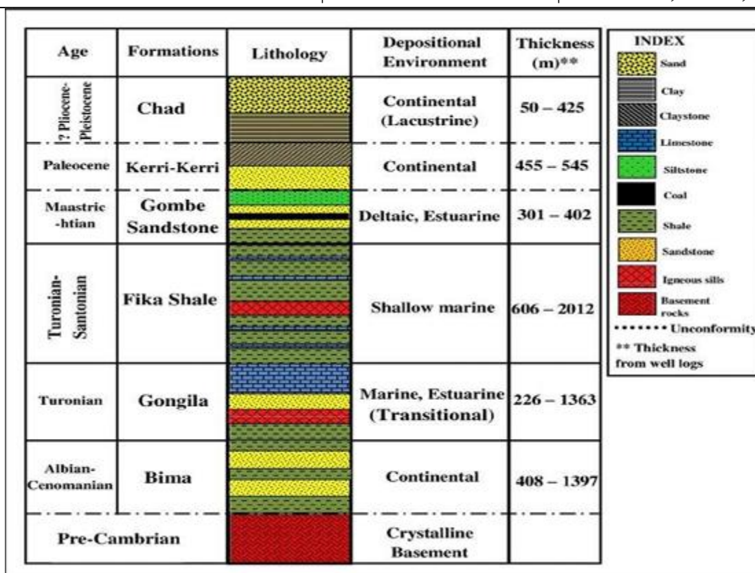
Figure 3. Stratigraphic data sheet of the Nigeria Chad Basin (after Okosun 1995; Avbovbo et al., 1986; Carter et al., 1963)
