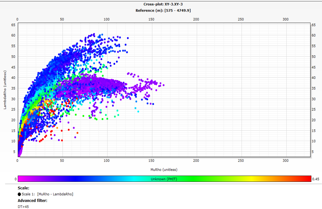
Figure 12: LambdaRho vs MuRho plot coloured by porosity
