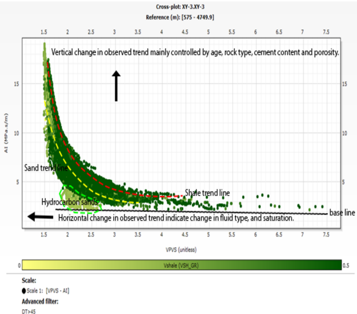
Figure 5: AI vs VPVS plot with trendline for sand and shale. Colour represents changing facies in terms of shaliness (volume of shale). The background masks the overall response making it difficult to identify the trend.
