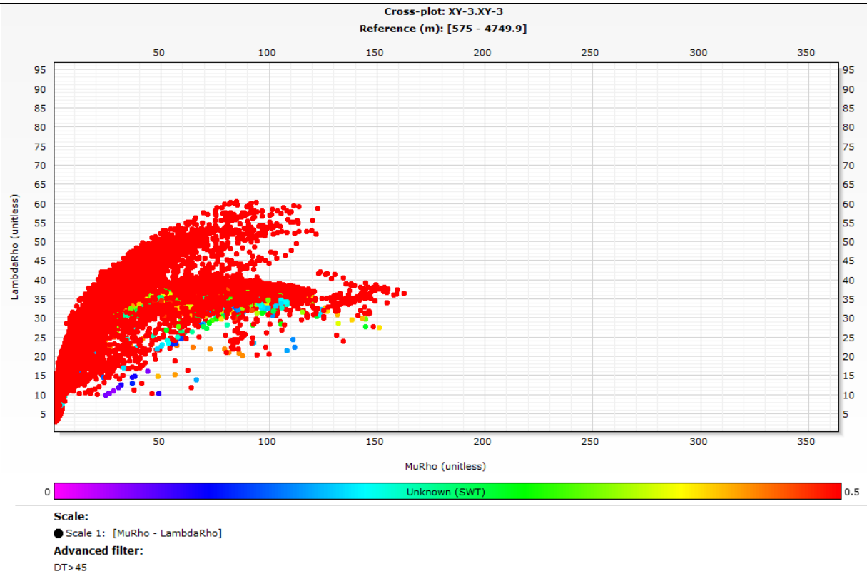
Figure 10: LambdaRho vs MuRho plot coloured by water saturation.
