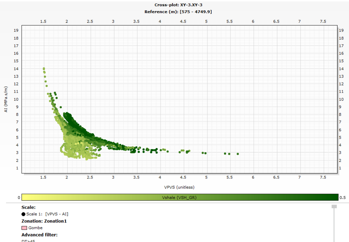
Figure 7: AI vs VPVS plot for the Gombe Formation reservoir interval.
