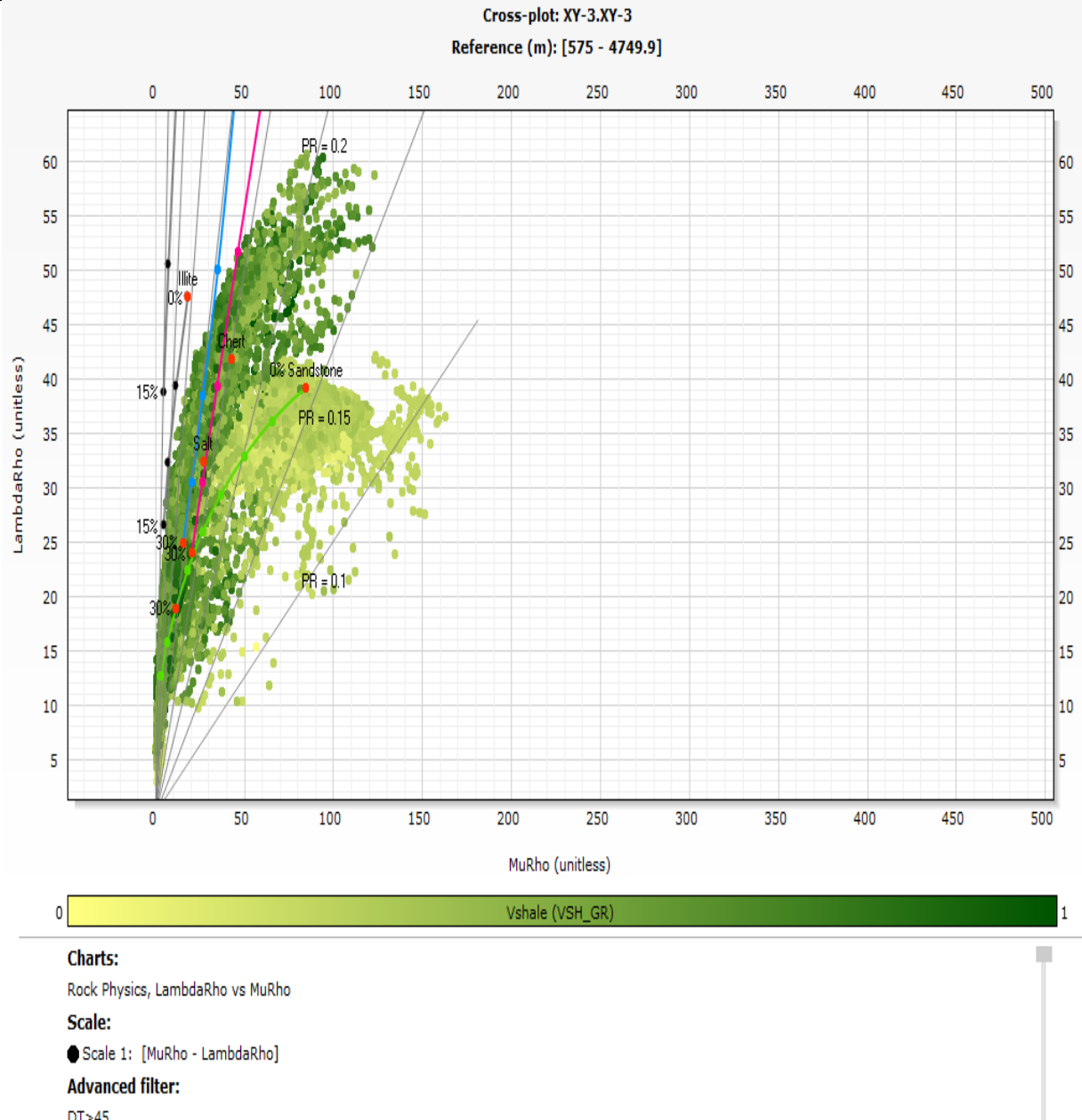
Figure 14: LambdaRho vs MuRho plot coloured by volume of shale with theoretical trendlines for lithology.
