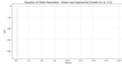
(a) Equation of state parameter
