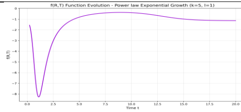
Figure 5. f(R,T) vs. time.
