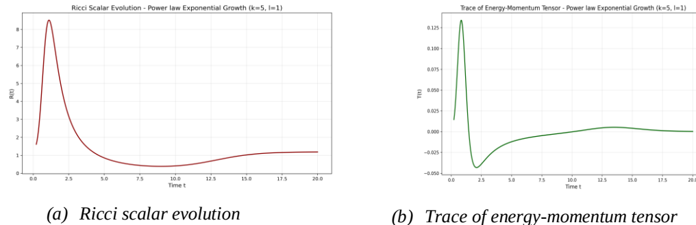
Figure 4 (a) Ricci scalar R(t) vs. time. (b) Trace of energy-momentum tensor T(t) vs. time.
