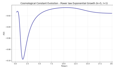
Figure 3. Cosmological constant evolution \Lambda(t) vs. time.
