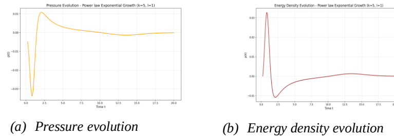
Figure 2 (a) Pressure evolution p(t) vs. time. (b) Energy density evolution \rho(t) vs. time.
