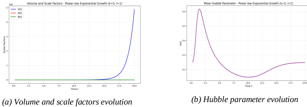
Figure 1. (a) Evolution V(t) and A(t) and B(t) vs. time. (b) Mean Hubble parameter H(t) vs. time.
