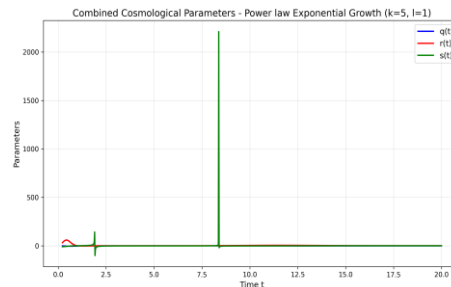
Figure 8. Combined evolution q(t) , r(t) and s(t) vs. time.
