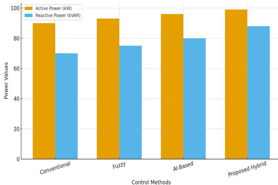
Fig. 2. Power Output Stability Across Load Variations
