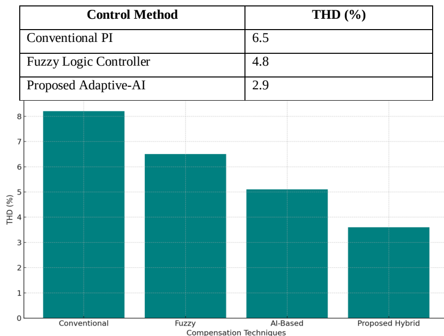
Fig. 3. Harmonic Distortion Comparison among Various Techniques
