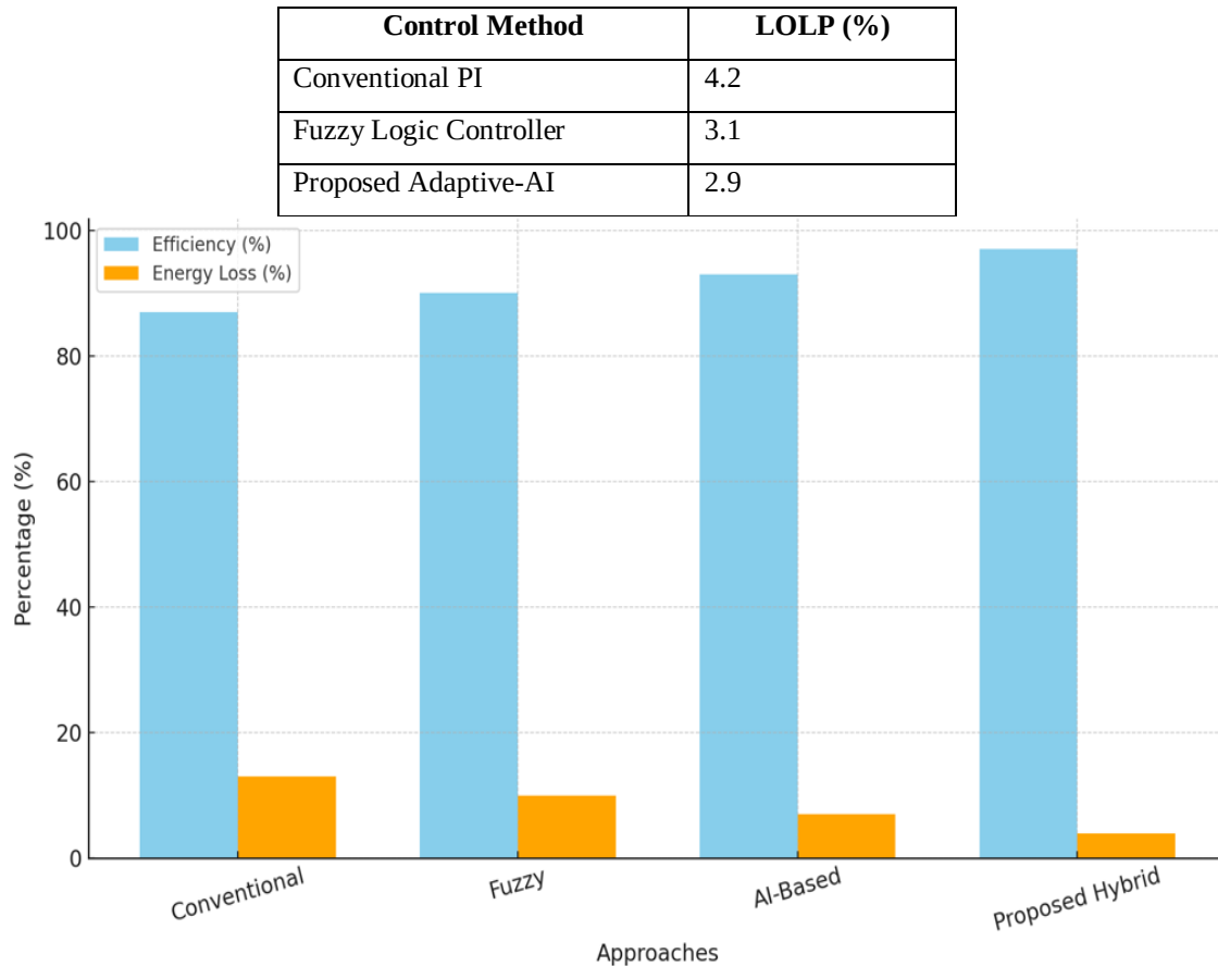
Fig. 5. Efficiency Benchmarking and Energy Loss Reduction
