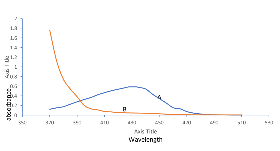
Fig.1 Absorption Spectrum of Ti (IV)-HTC complex Conditions: 2μg Ti(IV)/ml, other conditions are same as described in procedure
