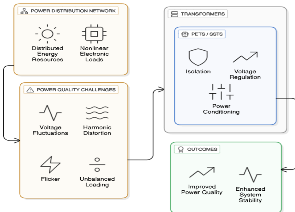
Fig. 1. Power Distribution Network Architecture
