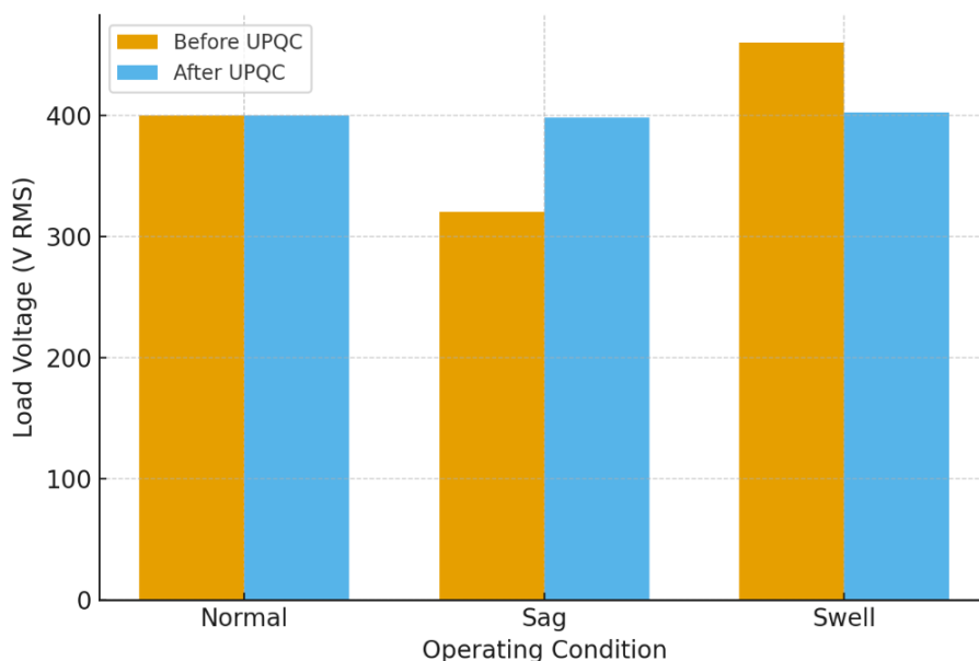
Fig. 2. Comparison of Load Voltage during Sag and Swell
