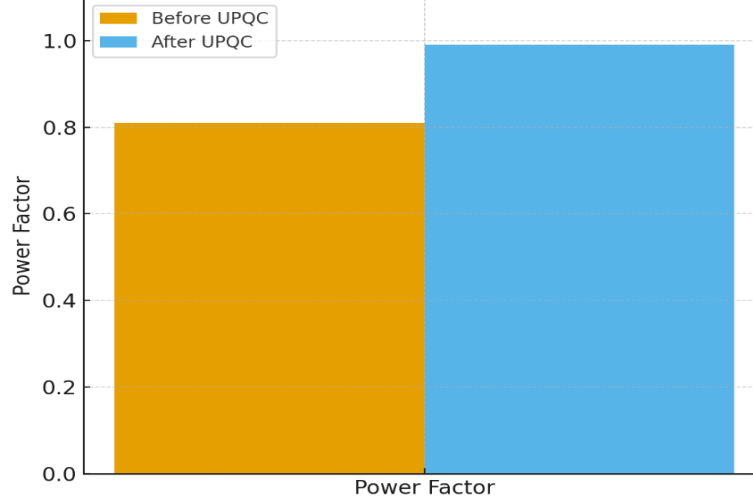
Fig. 4. Power Factor Improvement with UPQC
