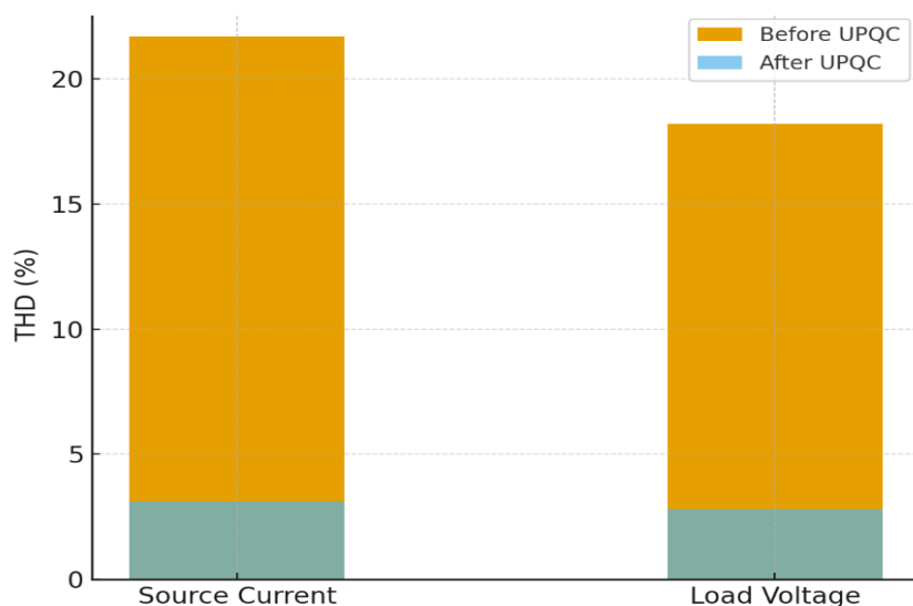
Fig. 3. THD Comparison before and after UPQC Operation
