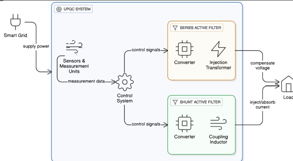
Fig. 1. Unified Power Quality Conditioner in Smart Grids
