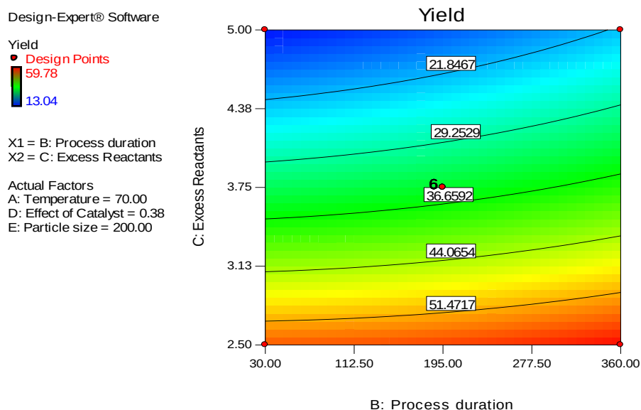
Figure 9: The contour plots for exces reactants against process duration and yield of ZAC
