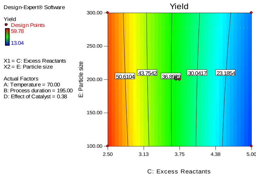
Figure 13: The contour plots for particle size against excess reactants and yield of ZAC
