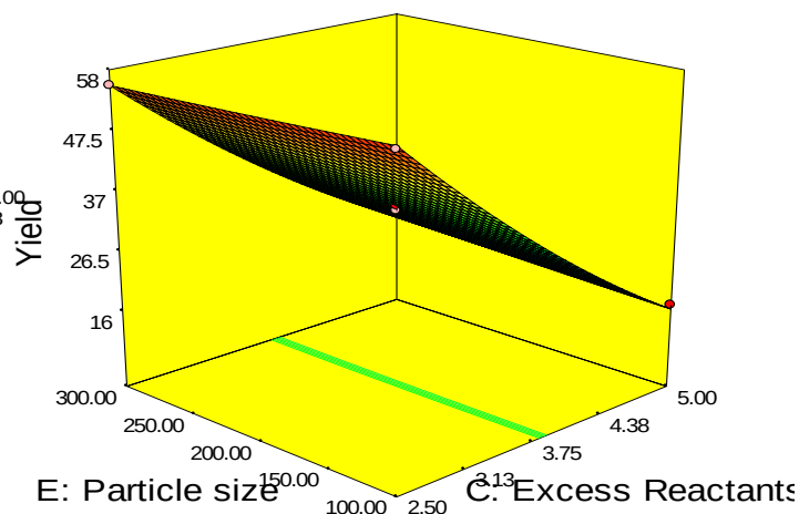
Figure 23: The 3 - D Plotfor particle size against excess reactants and yield of ZAC
