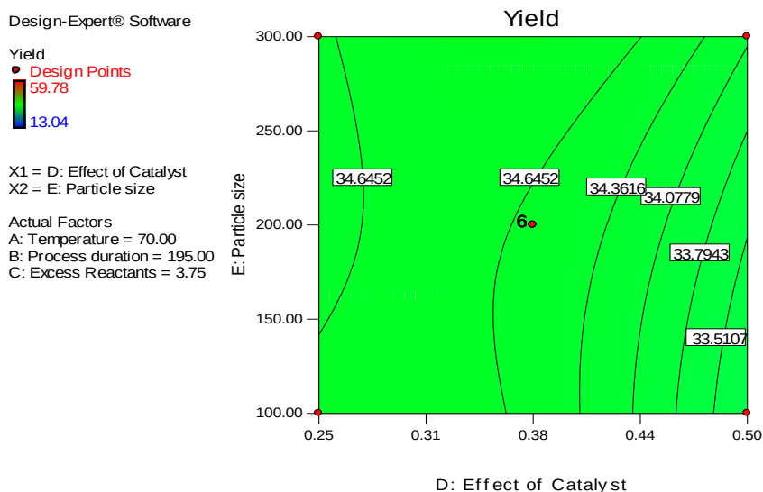
Figure 14: The contour plots for particle size against the effect of catalyst and yield of ZAC
