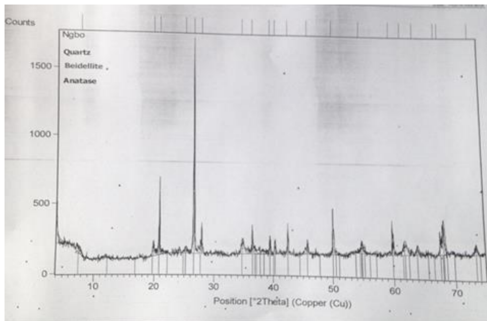
Figure 1: Results of XRD analysis of Ngbo raw clay
