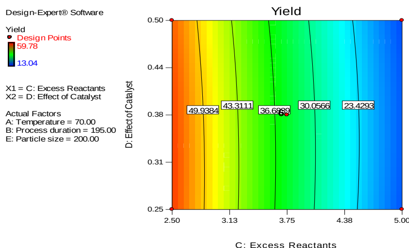
Figure 12: The contour plots for effect of catalyst against excess reactants and yield of ZAC
