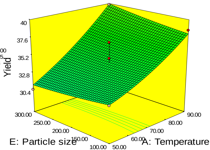
Figure 18: The 3 - D Plotfor particle size against temperature and yield of ZAC
