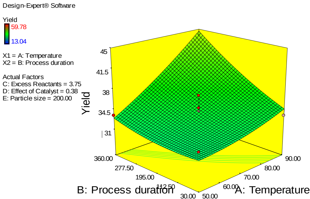
Figure 15: The 3 - D Plot for process duration against temperature and yield of ZAC
