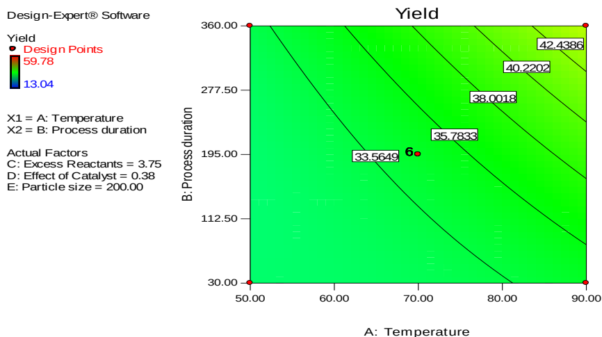
Figure 5: The contour plots for process duration against temperature and yield of ZAC
