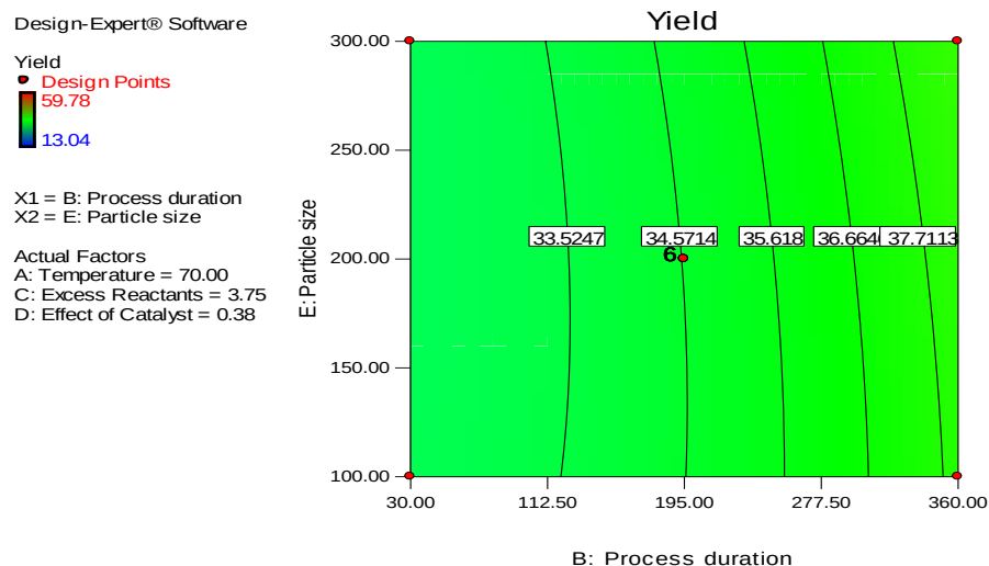
Figure 11: The contour plots for particle size against process duration and yield of ZAC
