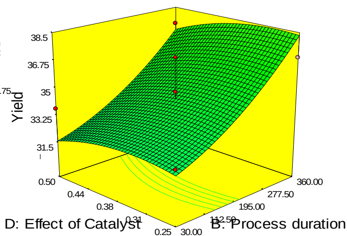
Figure 20: The 3 - D Plotfor effect of catalyst against process duration and yield of ZAC
