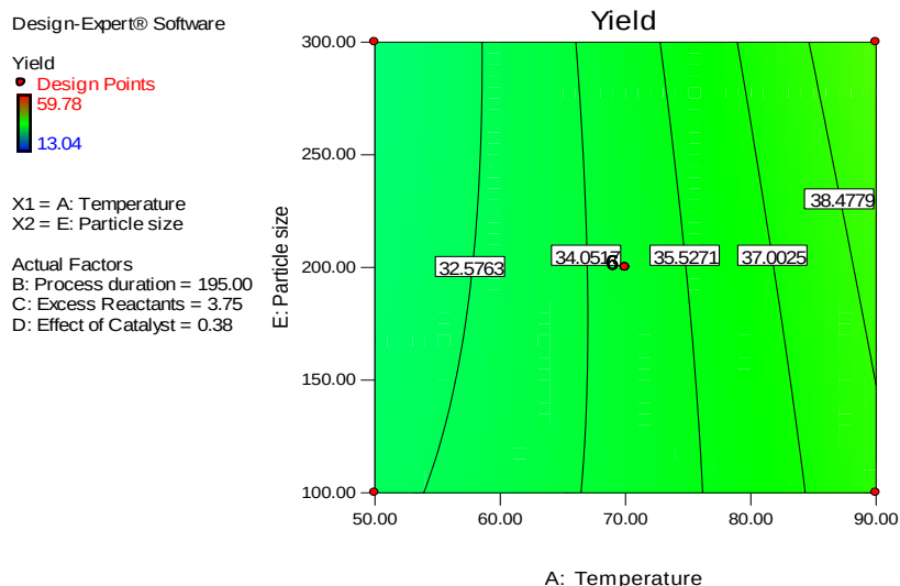
Figure 8: The contour plots for particle size against temperature and yield of ZAC
