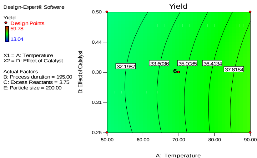
Figure 7: The contour plots for effect of catalyst against temperature and yield of ZAC
