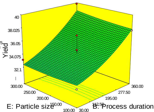
Figure 21: The 3 - D Plotfor particle size against process duration and yield of ZAC
