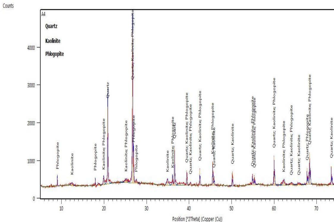
Figure 2: Results of XRD analysis of Zinc Chloride Activated Clay
