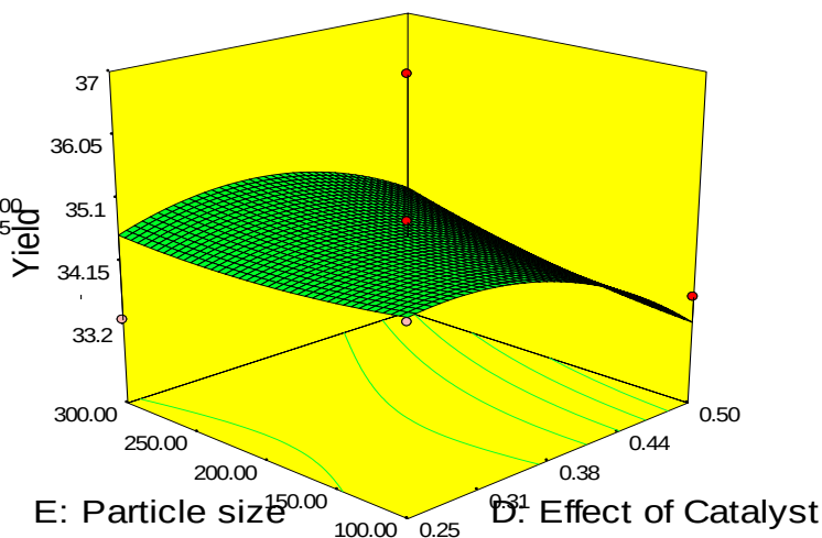
Figure 24: The 3 - D Plotfor particle size against effect of catalystand yield of ZAC
