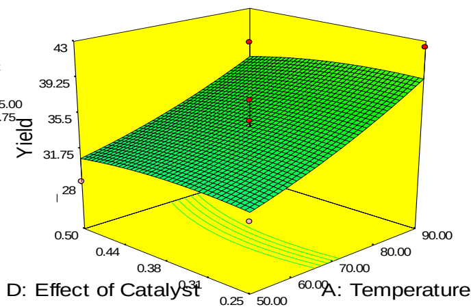
Figure 17: The 3 - D Plotfor effect of catalyst against temperature and yield of ZAC
