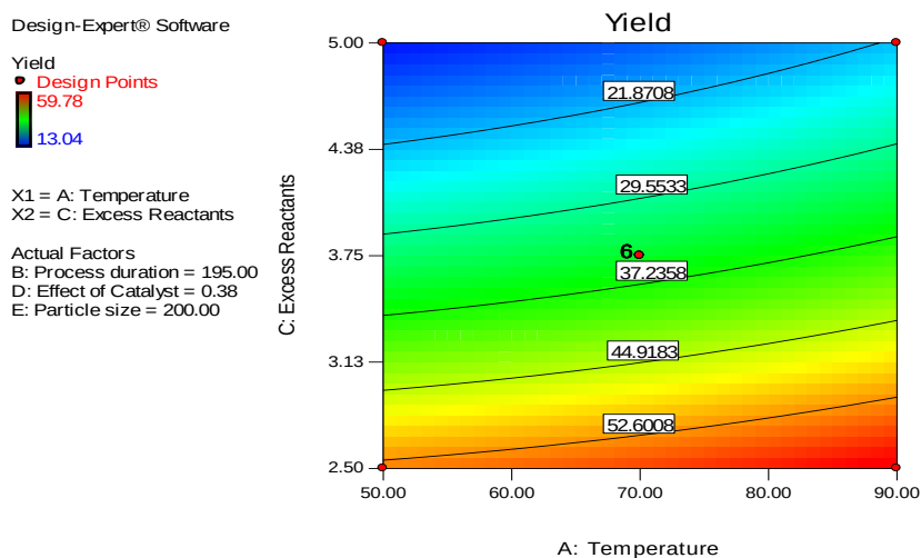
Figure 6: The contour plots for excess reactants against temperature and yield of ZAC
