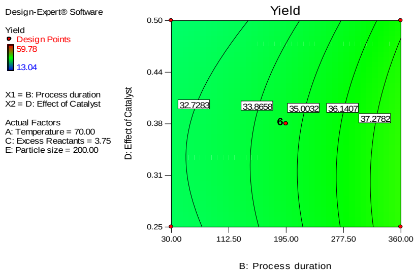
Figure 10: The contour plots for effect of catalyst against process duration and yield of ZAC
