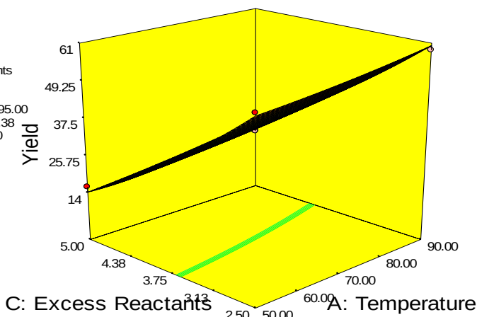
Figure 16: The 3 - D Plotfor excess reactants against temperature and yield of ZAC
