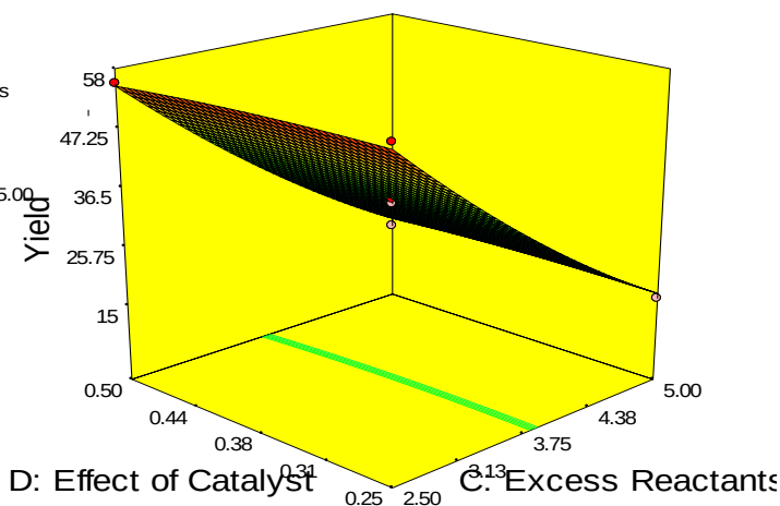
Figure 22: The 3 - D Plotfor effect of ctalyst against excess reactants and yield of ZAC
