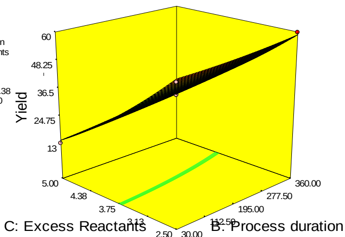
Figure 19: The 3 - D Plot for excess reactants against process duration and yield of ZAC
