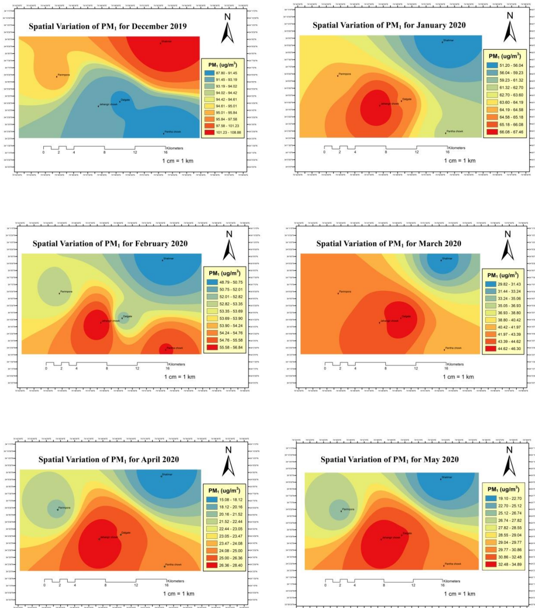
Figure 7: IDW maps showing variation in concentrations of pollutants ( PM_1 ) at different locations during each month from June 2019 to May 2020.
