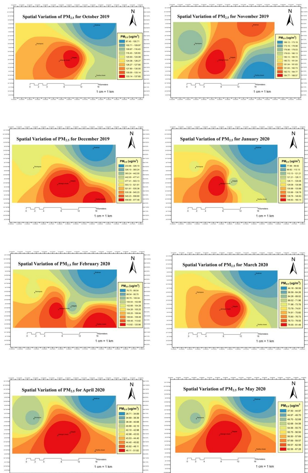
Figure 8: IDW maps showing variation in concentrations of pollutants (PM 2.5 ) at different locations during each month from June 2019 to May 2020.
