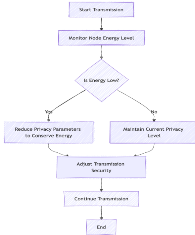
Flowchart for Adaptive Privacy Parameter Change Mechanism (A2PCM)
