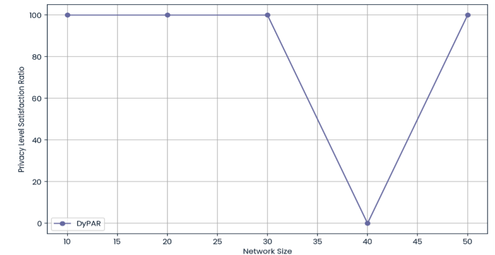
Privacy Level Satisfaction Ratio (PLSR) vs Network Size
