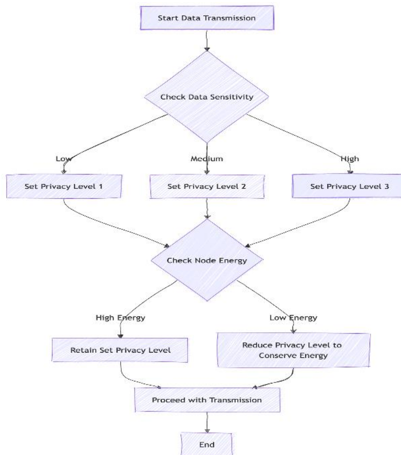
Flow chart for DyPAR
