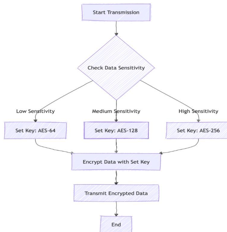
DyPAR Efficient Key Management Flow Chart
