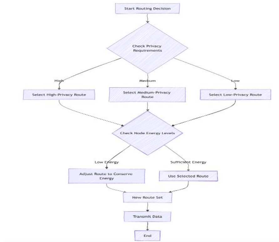
Dynamic Routing Decisions (DyRD) Flow chart
