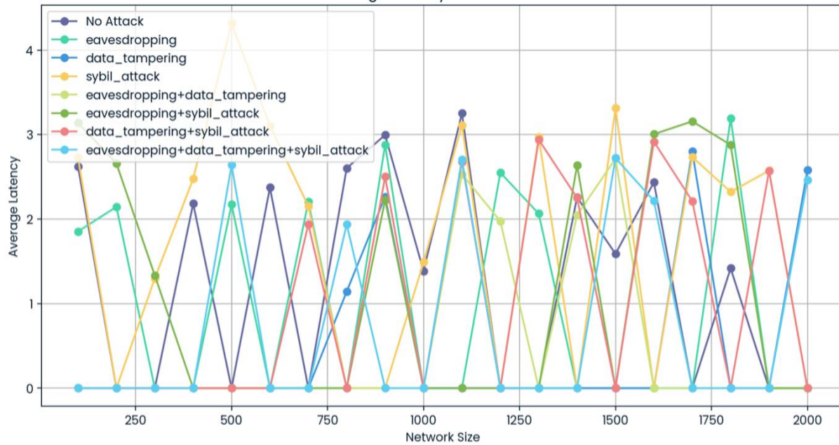
Average Latency vs Network Size
