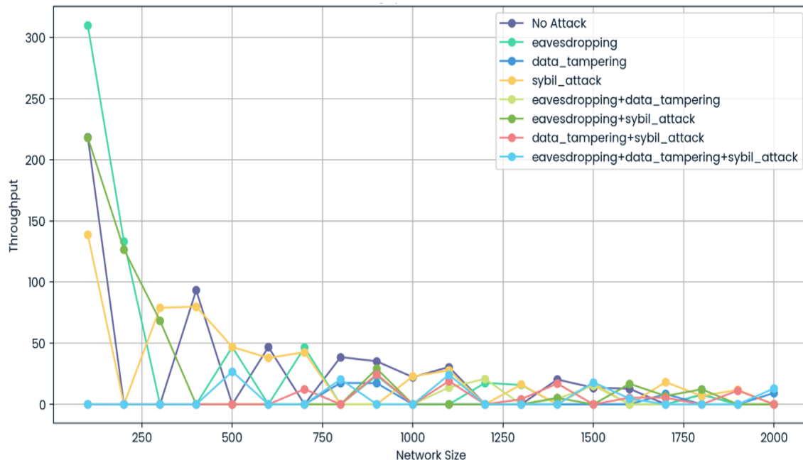
Throughput vs Network Size
