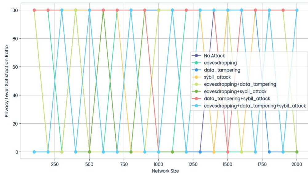
Privacy Level Satisfaction Ratio (PLSR) vs Network Size
