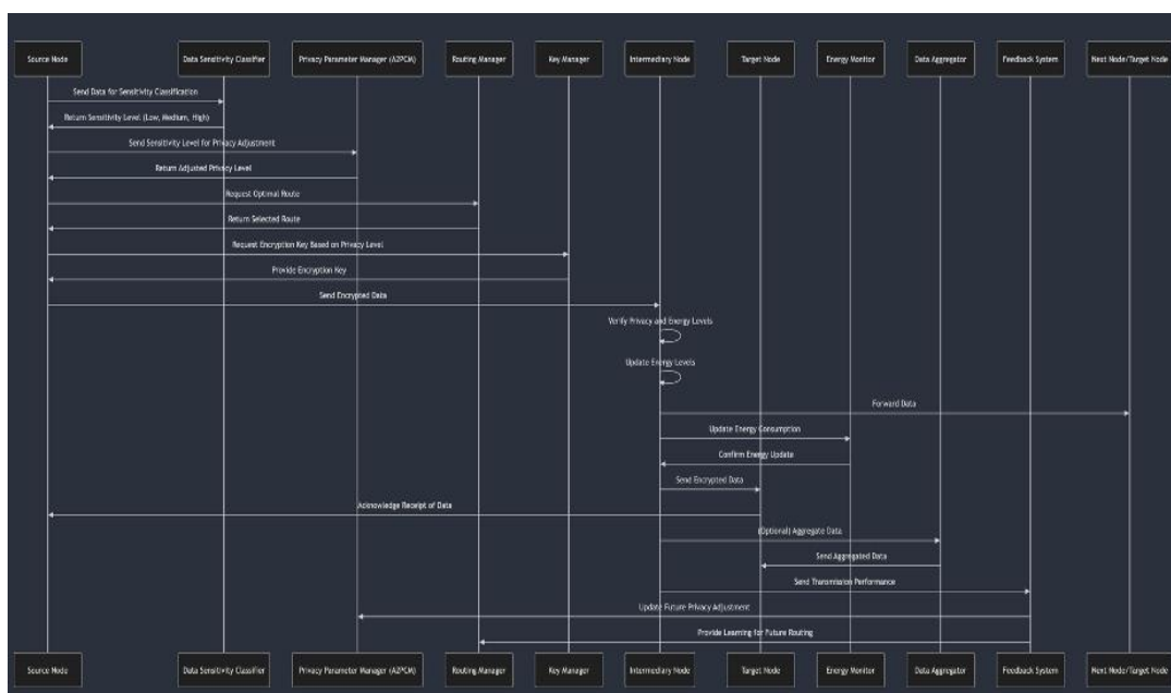
Sequence Diagram for DyPAR
