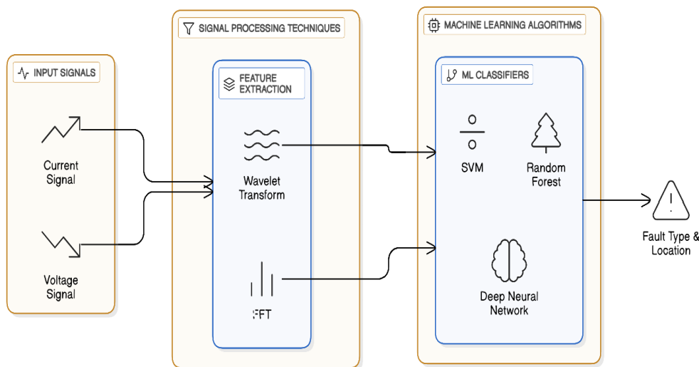
Fig. 1. Integrated Framework for Power System Fault Detection
