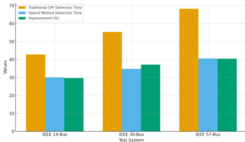
Fig. 2. Comparison of Fault Detection Time Between Traditional CPF and Hybrid Method
