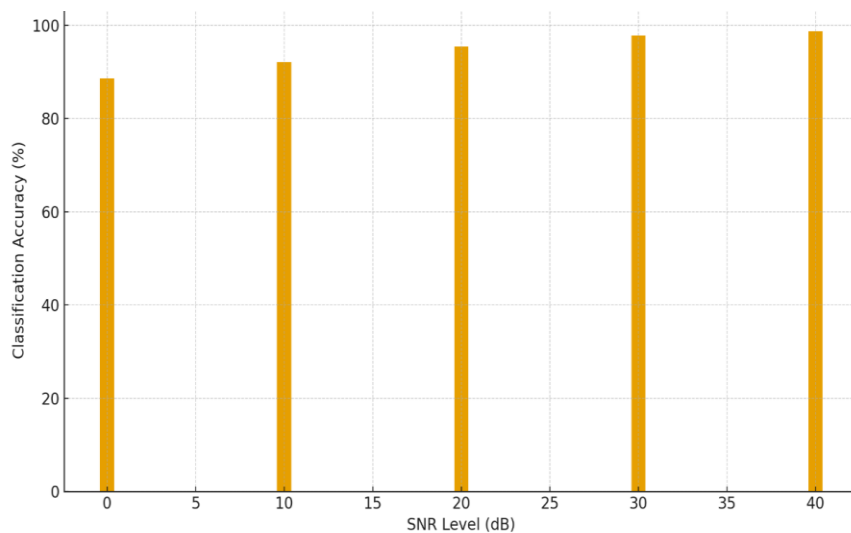
Fig. 3. DNN Classification Accuracy Under Different SNR Levels
