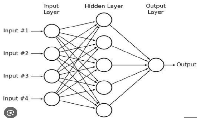
Figure 7: Multi-layer Perceptron ( https://www.futurelearn.com/ )
