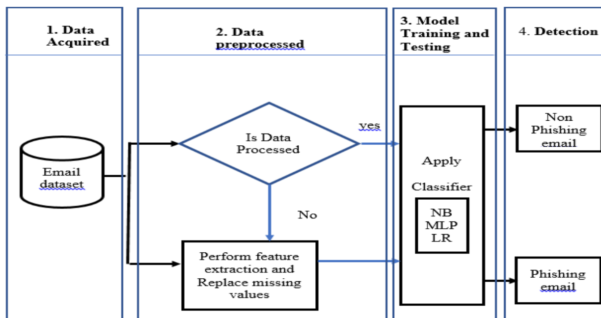
Figure 1: Flow diagram of the system (Author, 2025)
