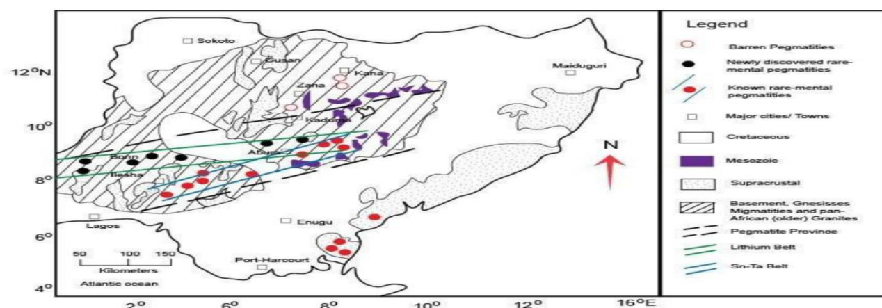
Figure 1: The Lithium and Tantalum Belts in Nigeria's Pegmatite Province (Isa et al., 2024)
