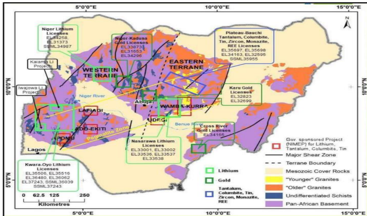
Figure 2: Geological Map of Nigeria Showing Major Rock Groups (MMSD, 2022)
