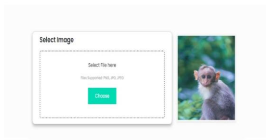
Fig. 12. Prediction result
