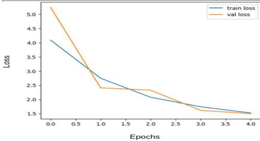
Fig. 2. Training and validation loss graph of CNN
