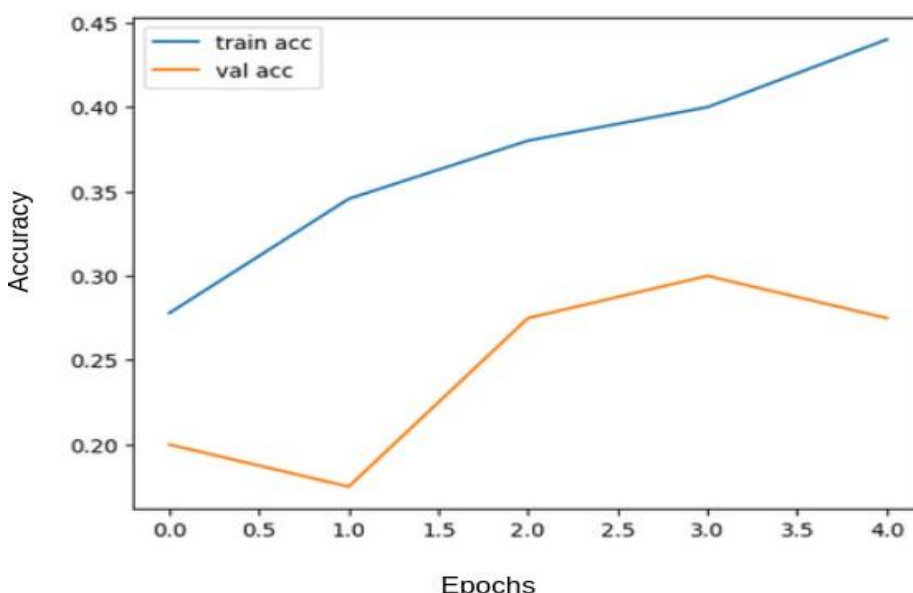
Fig. 1. Training and validation accuracy graph of CNN
