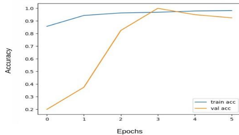
Fig. 3. Training and validation accuracy graph of ResNet 50
