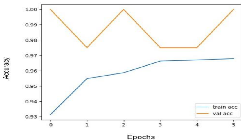
Fig. 5. Training and validation accuracy graph of Inception v3
