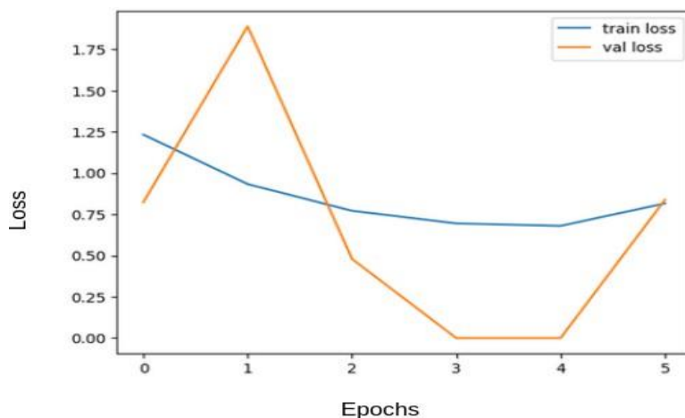
Fig. 14. Training and validation loss graph of final model
