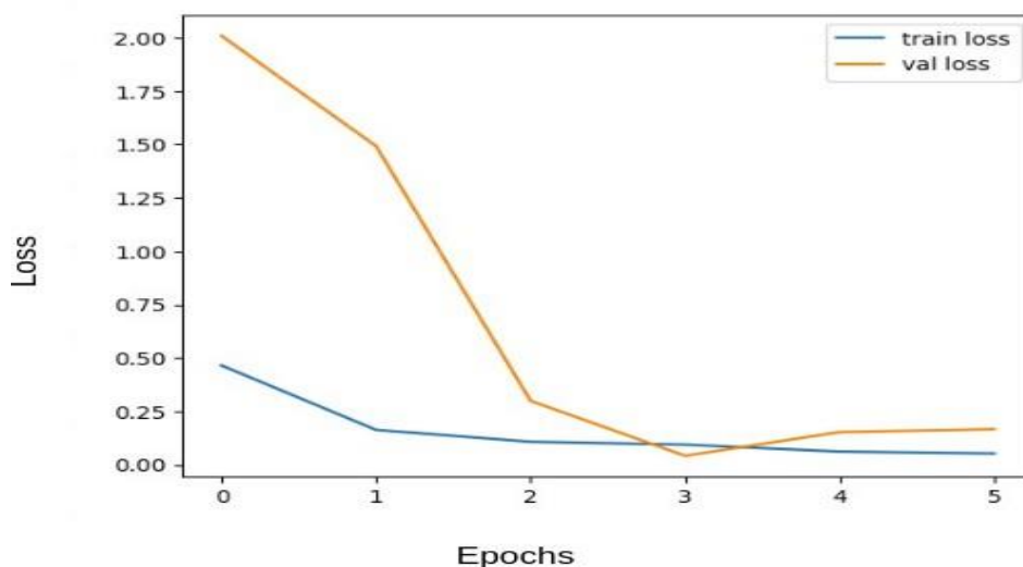
Fig. 4. Training and validation loss graph of ResNet 50
