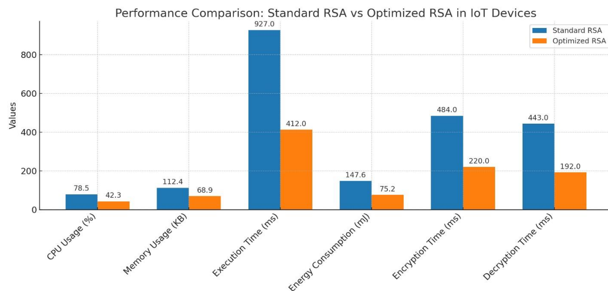
Figure 4.1: Execution time comparison between standard RSA and optimized RSA.
