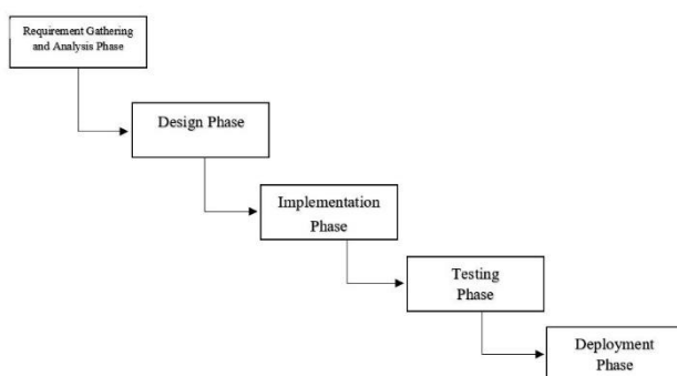
Fig. 3 Waterfall Model
