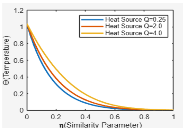
Figure 10 In Fig. 10, the temperature goes up because greater Heat source (Q) contributes more thermal energy to the fluid, which makes it hotter.
