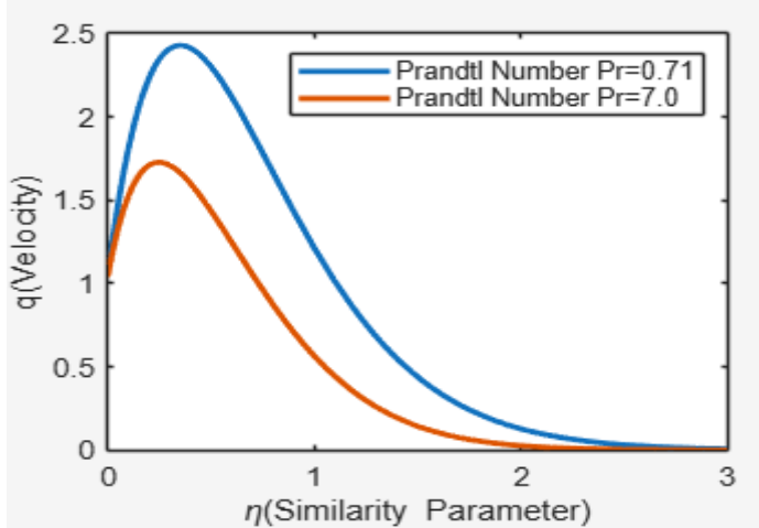
Figure 8 In Fig 8 As the Prandtl number (Pr) goes up, the velocity (speed) goes down. This is because a higher Prandtl number indicates that momentum spreads out quicker than heat, which slows down the fluid motion and stops the thermal boundary layer from growing.
