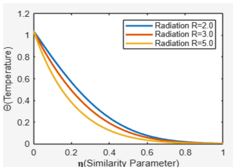
Figure 9 In Fig 9 As radiation (R) rises, the temperature drops. This is because increased radiation takes heat out from the fluid, lowering its thermal energy and lowering the temperature.
