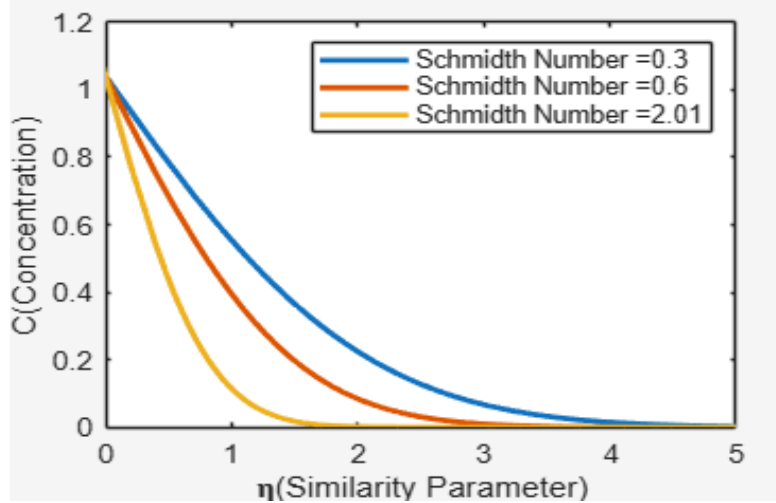
Figure 11 In Fig 11 The Schmidt number ( Sc ) goes up, which means that mass diffusion is slower than momentum. This slows down the flow and diminishes the fluid motion.
