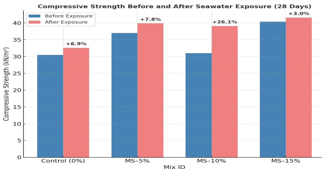
Figure 5.1 Variation of Compressive Strength before and after Seawater Exposure (28 Days)
