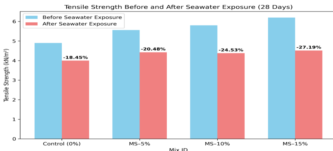
Figure 5.2 Variation of Tensile Strength before and after Seawater Exposure (28 Days)
