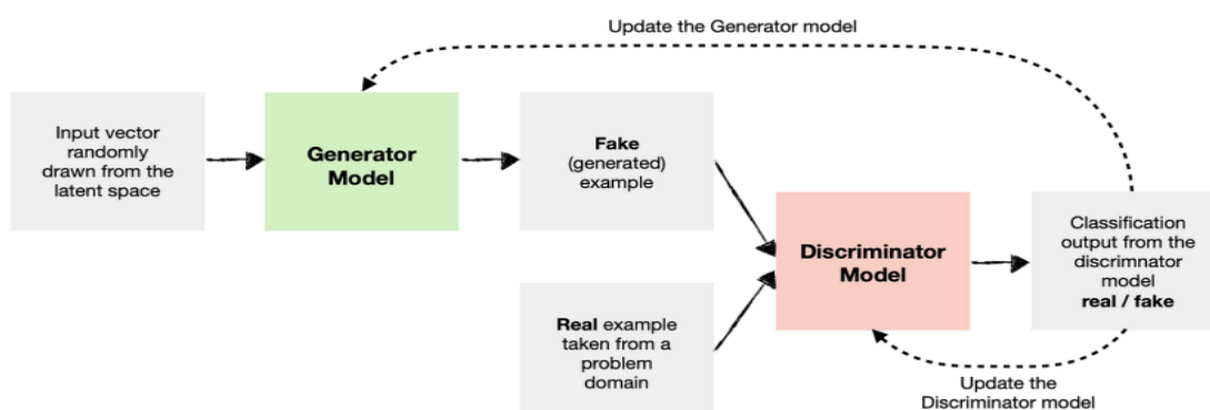
Figure 3. Proposed GAN workflow
