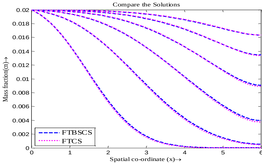
Figure 4.3: Concentration distribution profiles of CDE with \Delta x = 0.05 , \Delta t = 0.1 pe < 1
