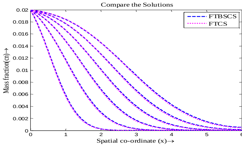
Figure 4.1: Concentration distribution profiles of CDE with \Delta x = 0.05 , \Delta t = 0.033 , pe \ll 1
