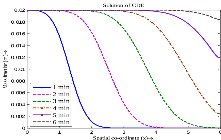
Figure 5.1: Solution of CDE by FTBSCS at different time with v=0.01 \text{ m}^2/\text{s} and D=0.001 \text{ m}^2/\text{s} .
