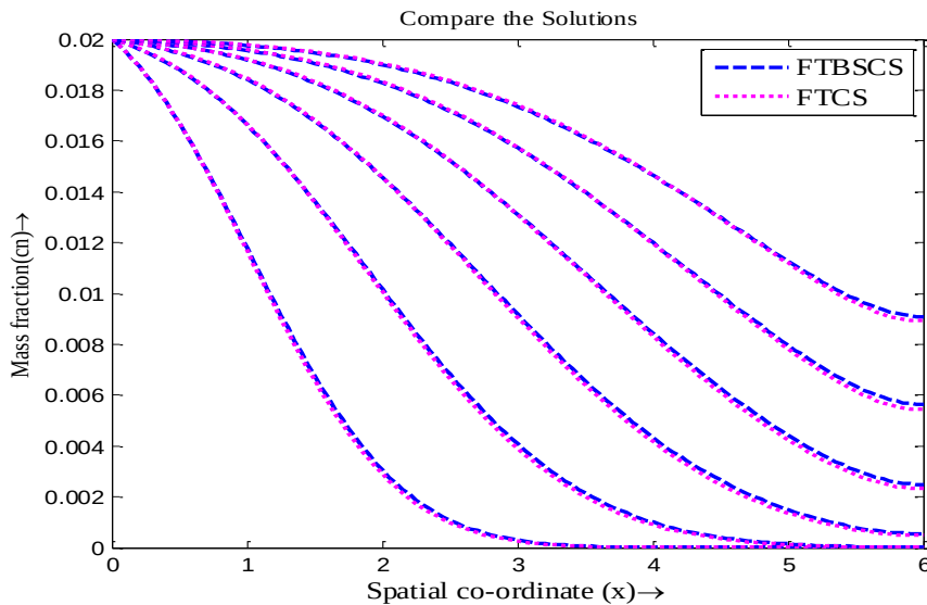
Figure 4.2: Concentration distribution profiles of CDE with \Delta x = 0.05 , \Delta t = 0.067 pe \ll 1
