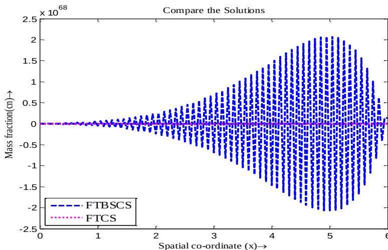
Figure 4.5: Concentration distribution profiles of CDE with \Delta x = 0.05 , \Delta t = 0.122 pe \approx 1
