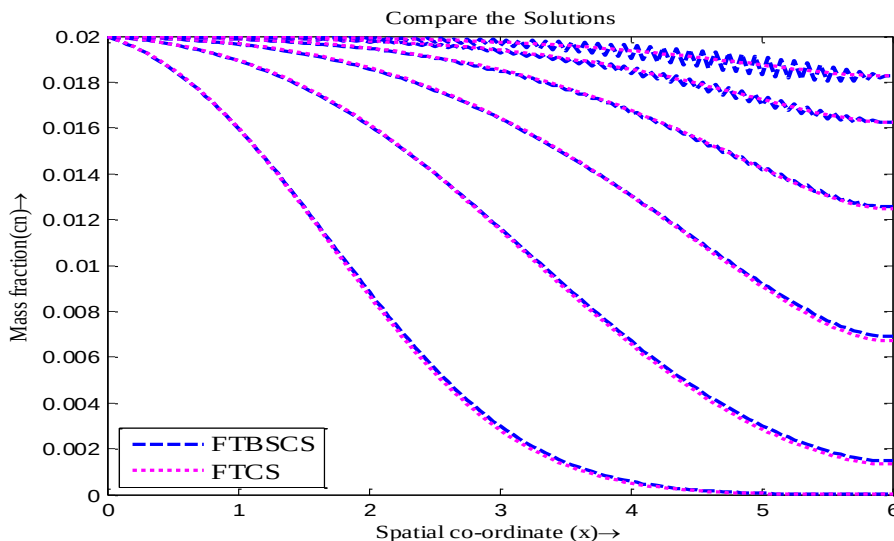
Figure 4.4: Concentration distribution profiles of CDE with \Delta x = 0.05 , \Delta t = 0.1192 , pe \approx 1
