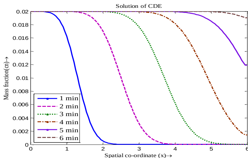
Figure 5.2: Solution of CDE by FTCS at different time with v=0.01 \text{ m}^2/\text{s} and D=0.01 \text{ m}^2/\text{s} .
