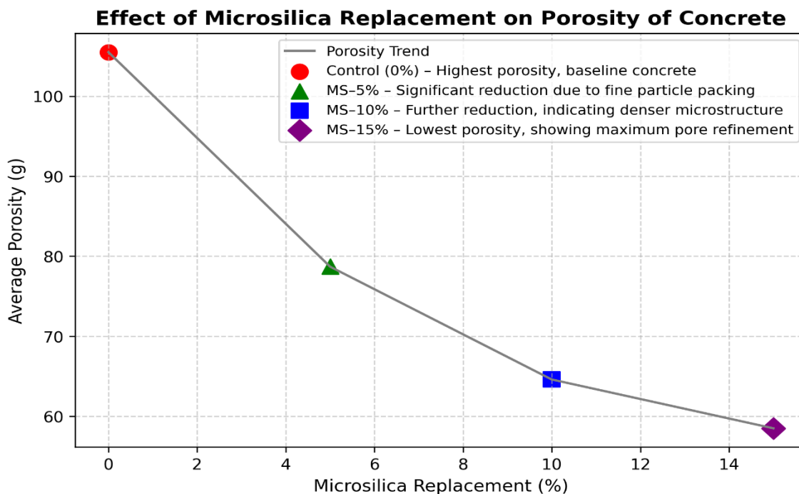
Figure 4.7 Average Porosity of Concrete with Partial Replacement of Cement by Microsilica
