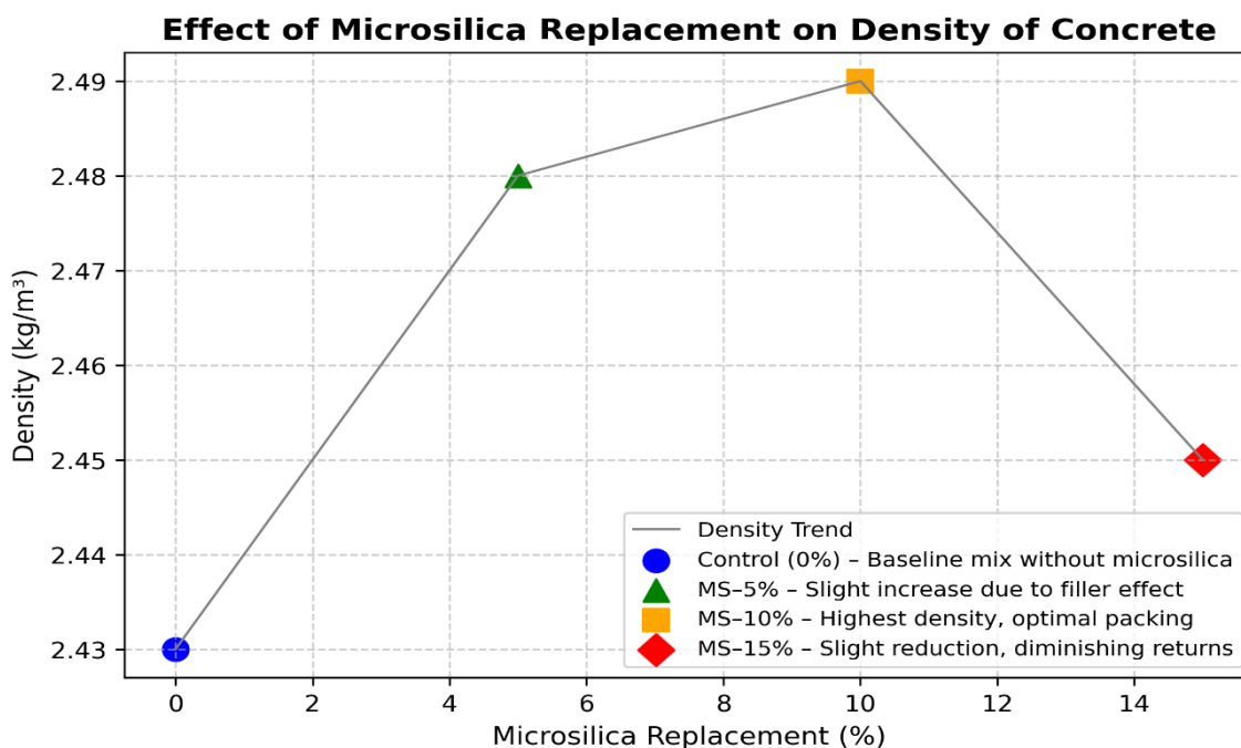
Figure 4.6 Average density of concrete with partial replacement of cement by microsilica.
