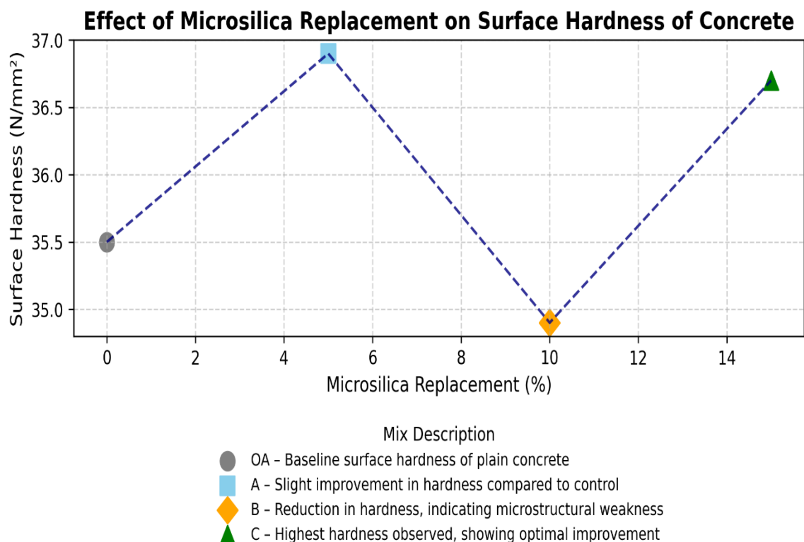
Figure 4.8 Average Surface Hardness Of Concrete With Partial Replacement Of Cement By Microsilica.
