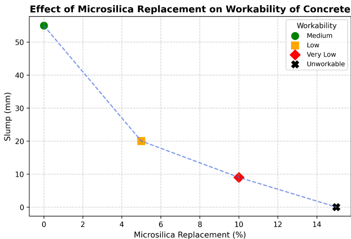
Figure 4.5 Average Workability (Slump) Of Concrete With Partial Replacement Of Cement By Microsilica.
