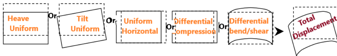
Fig. 3: The causes of foundation failure that result in structural collapse in India
