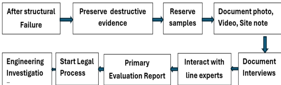
Fig. 1: The procedures to be followed by a Forensic Engineer after a building collapse.
