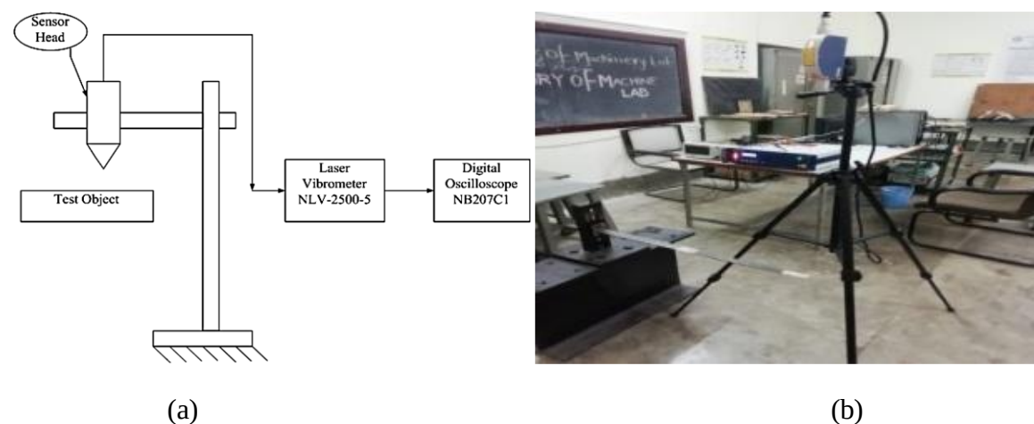
Fig. 2. (a) Basic and (b) actual experimental set-up.
