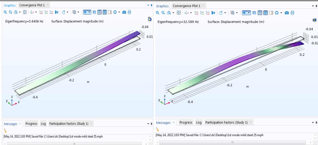
Fig. 4. Natural frequency of C-F M.S. non-uniform beam and corresponding mode shapes by simulation
