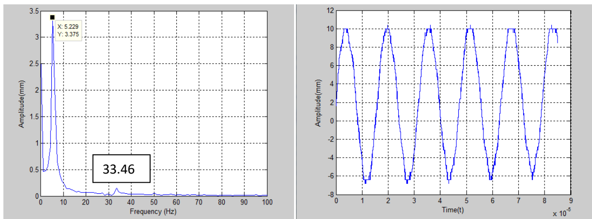
Fig. 3. Frequency domain and Time domain signals for non-uniform M.S. beam
