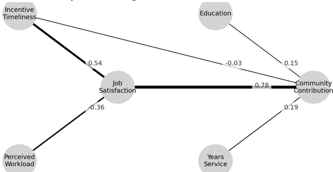
SEM-style Path Diagram (standardized coefficients)
