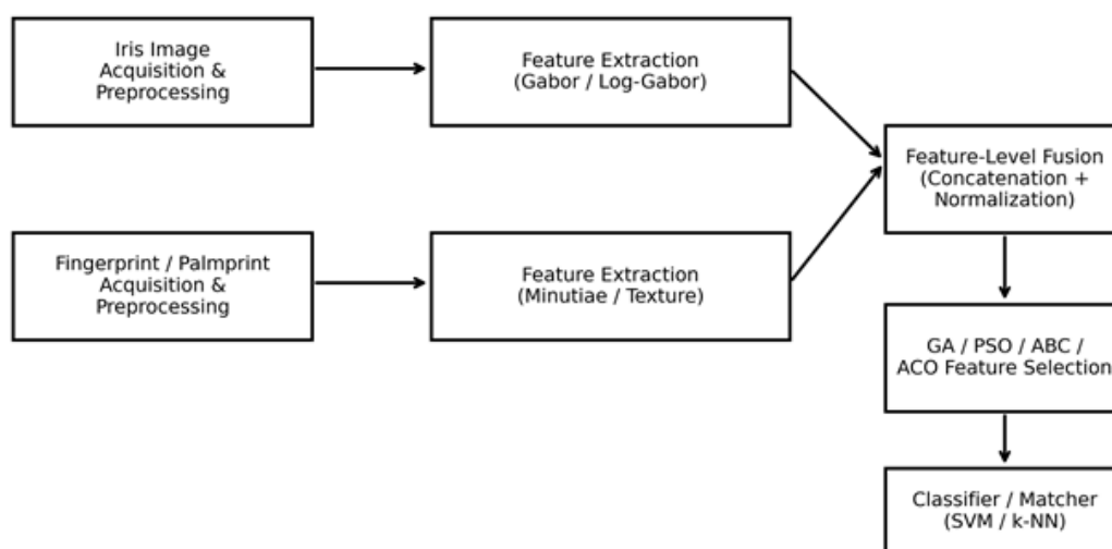
Fig. 6.1 Feature-level fusion based multimodal biometric recognition framework with swarm and evolutionary feature selection.
