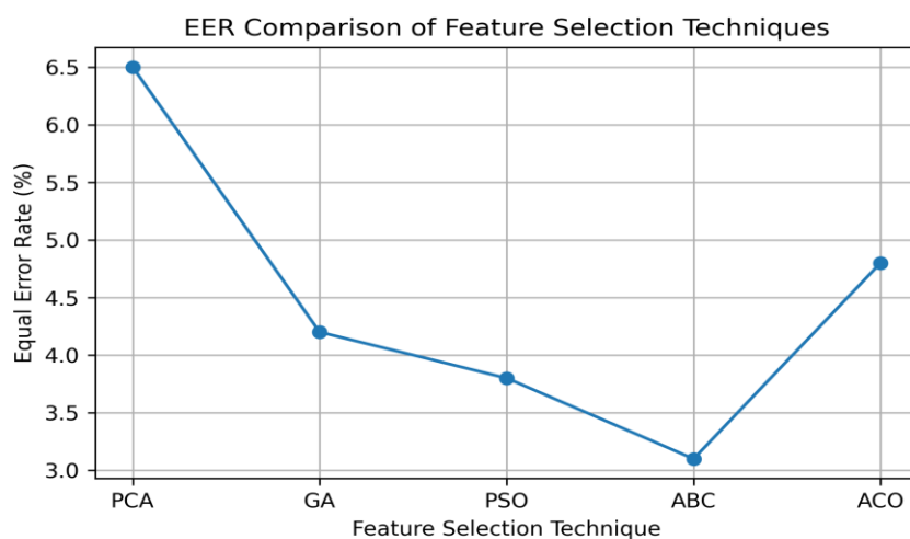
Fig 7.2: EER Comparison of Feature Selection Techniques
