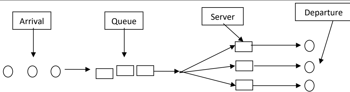
Fig 2.2: A multiple server queuing system, M/M/C
