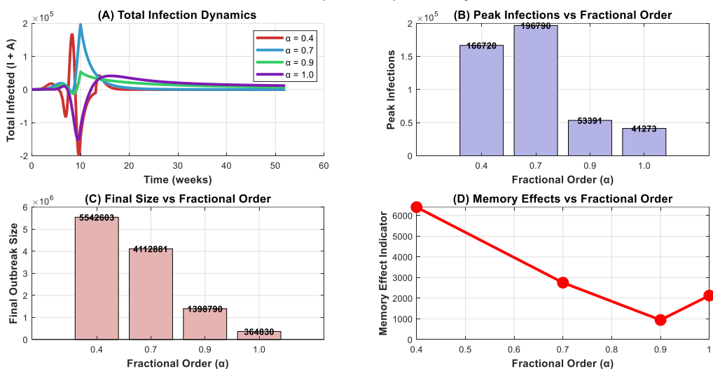
Fractional Order Impact on Diphtheria Dynamics
