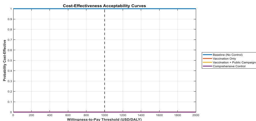
Figure 5(b): Cost-effectiveness acceptability curve using fitted parameter values in Table 3.
