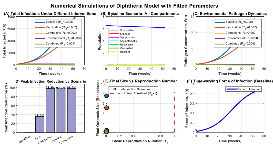
Figure 6: Numerical simulation for the diphtheria model (1) showing the Pictorial (A) Total infections under different interventions, (B) Baseline scenario: all compartments, (C) Environmental pathogen dynamics, (D) Peak infection reduction by scenario, (E) Final size vs reproduction number, and (F) Time varying force of infection (baseline), using fitted parameter values in Table 3.
