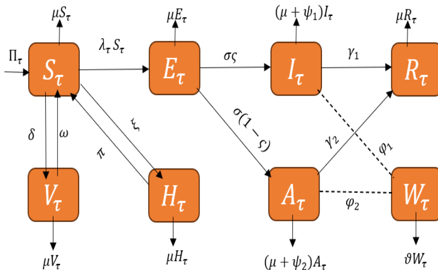
Figure 1: The model's schematic flow diagram (1)
