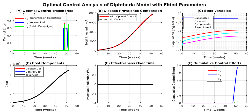
Figure 4: Optimal control analysis for the diphtheria model (1) showing the Pictorial (A) Optimal control trajectories, (B) Disease prevalence comparison, (C) state variables, (D) cost components, (E) Effectiveness over time, and (F) Cumulative control efforts using fitted parameter values in Table 3.
