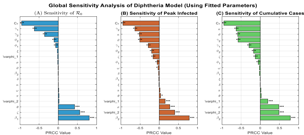
Figure 3: Global Sensitivity analysis of diphtheria model (1) via the partial rank correlation coefficient (PRCC) (A) showing the Pictorial Sensitivity of R_0 , (B) showing the Pictorial Sensitivity of peak infected, and (C) showing the Pictorial Sensitivity of cumulative cases using fitted parameter values in Table 3.
