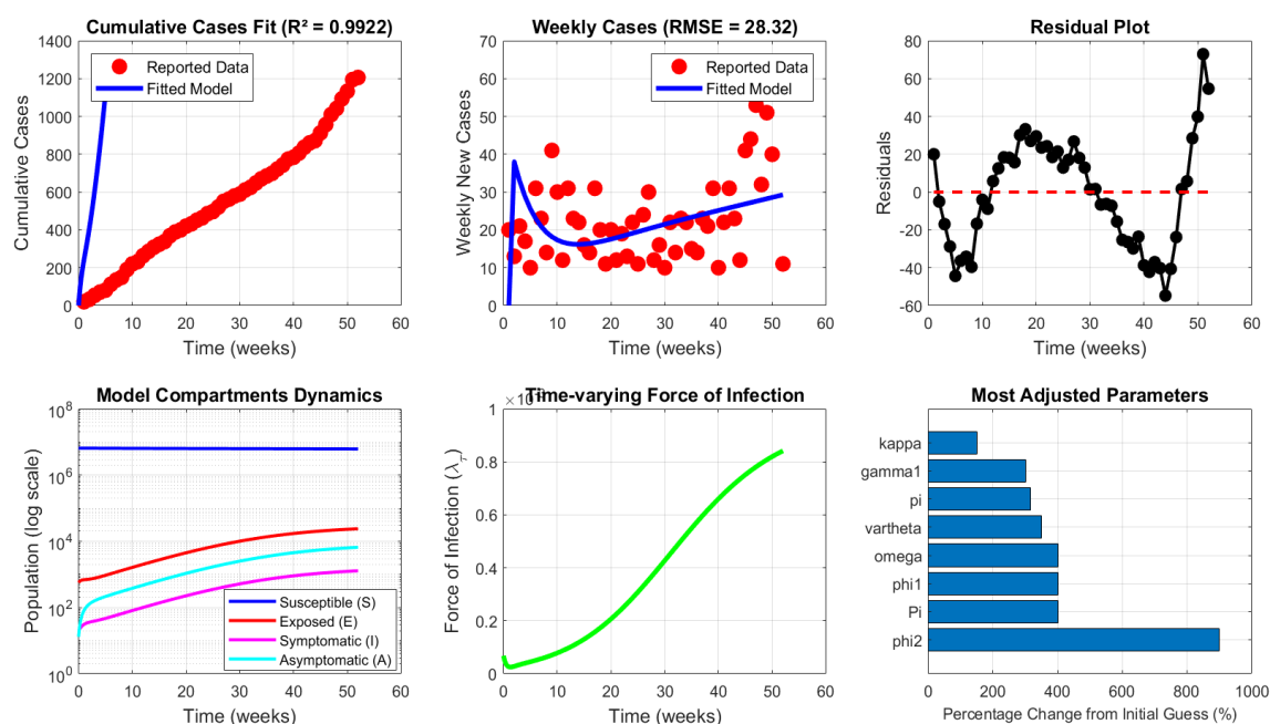
Figure 2: Model (1) data fitting of the diphtheria using cumulative confirmed incidence cases from Bauchi State, Northeast Nigeria, for the period from January to December 2023
