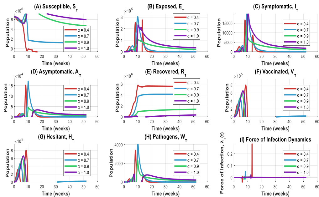
Caputo-Fabrizio Fractional Diphtheria Model: State Variable Dynamics
