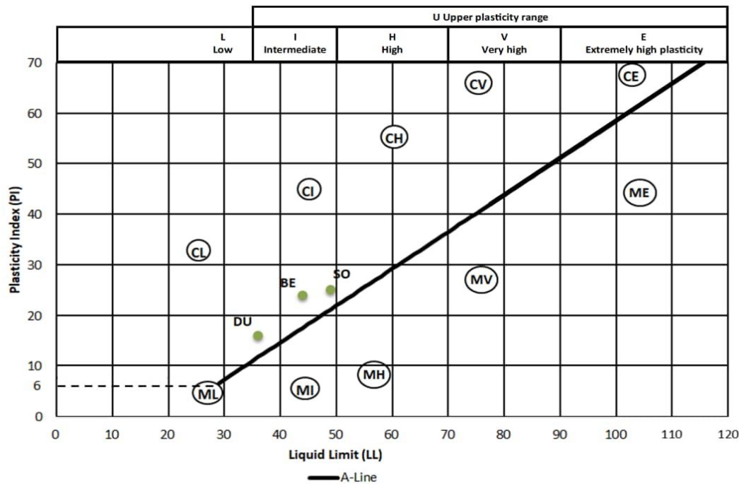
Figure 3: Plasticity of the Soils
