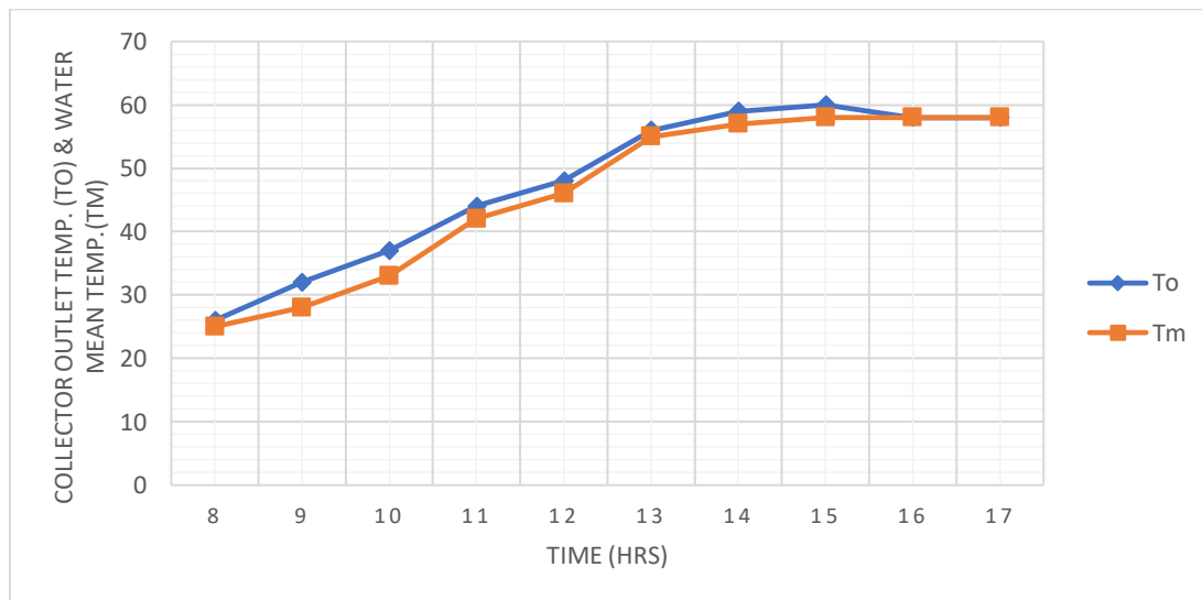
Fig. 1: graph of collector outlet temperature ( T_o ^{\circ}\text{C} ) & water mean temperature ( T_m ^{\circ}\text{C} ) against time (hrs) for Day 1
