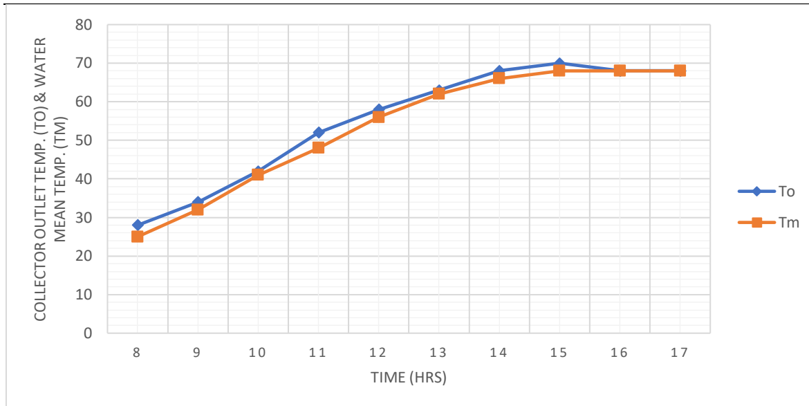
Fig. 6: Graph of collector outlet temperature ( T_o °C) & water mean temperature ( T_m °C) against time (hrs) for Day 6
