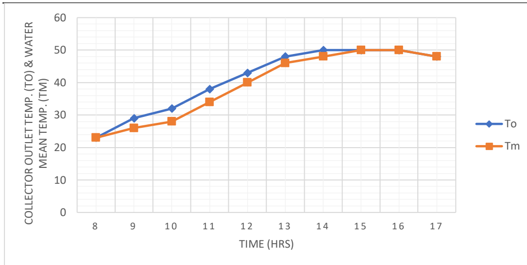
Fig. 3: graph of collector outlet temperature ( T_o °C) & water mean temperature ( T_m °C) against time (hrs) for Day 3
