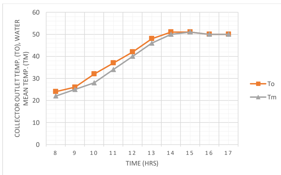
Fig. 4: graph of collector outlet temperature ( T_o °C) & water mean temperature ( T_m °C) against time (hrs) for Day 4
