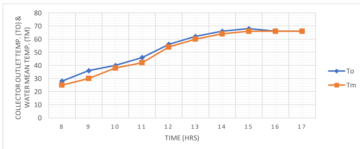
Fig. 5: graph of collector outlet temperature ( T_o °C) & water mean temperature ( T_m °C) against time (hrs) for Day 5
