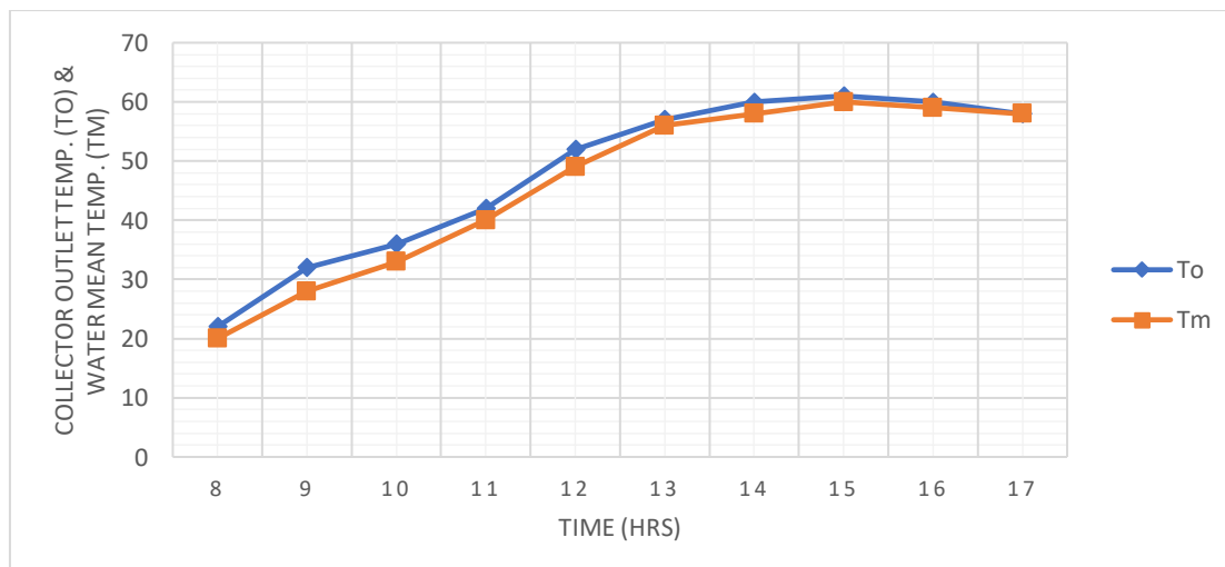
Fig. 2: graph of collector outlet temperature ( T_o ^{\circ}\text{C} ) & water mean temperature ( T_m ^{\circ}\text{C} ) against time (hrs) for Day 2
