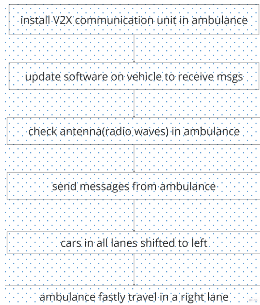
Fig 3: Deployment Workflow
