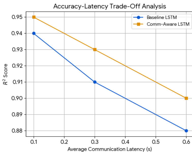
Figure 7. Accuracy–latency trade-off analysis
