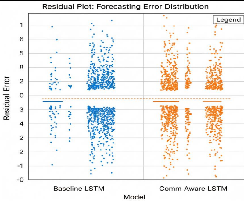
Figure 6: Error Distribution Comparison between Models
