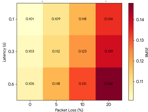
Figure 4: RMSE Heatmap under Communication Impairments
