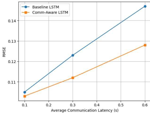
Figure 3. RMSE versus communication latency
