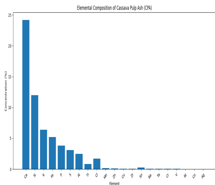
Figure 2: Elemental composition of CPA
