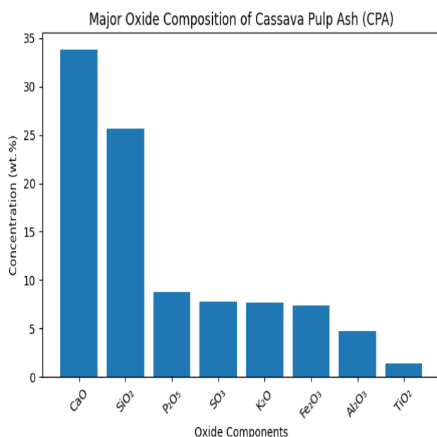
Figure 1: Major oxide composition of CPA
