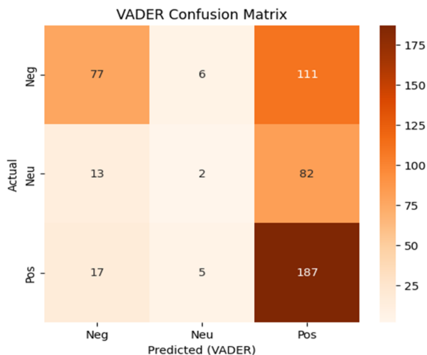
Figure 2. Confusion matrix for VADER sentiment classification
