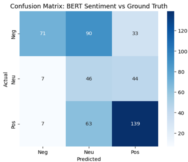
Figure 3. Confusion matrix for BERT-based sentiment classification
