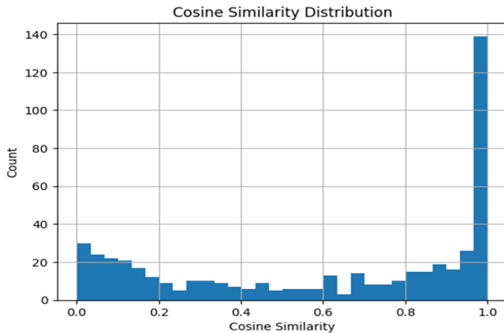
Figure 5. Cosine similarity distribution for BERT predictions
