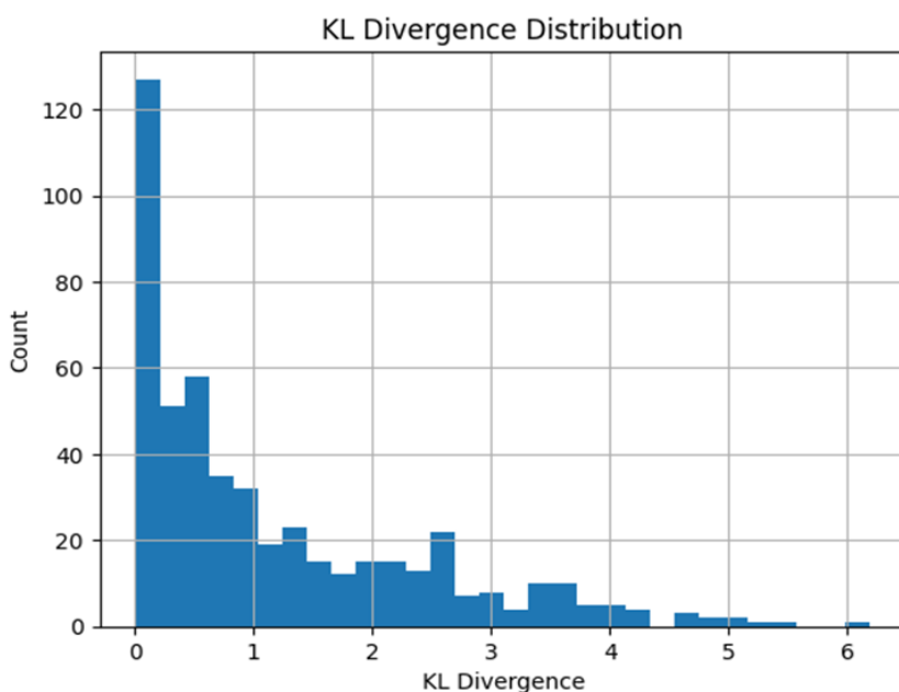
Figure 4. KL divergence distribution for BERT predictions
