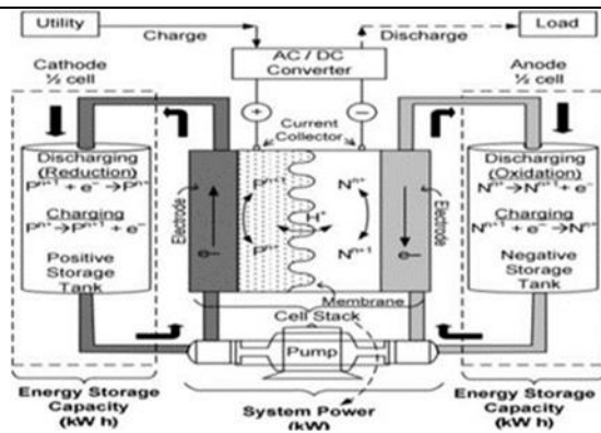
Figure 6: Typical diagram of a flow battery
