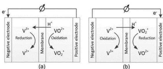
Figure 5: Schematic diagram of a vanadium redox flow battery: (a) charging reaction and (b) discharging reaction.
