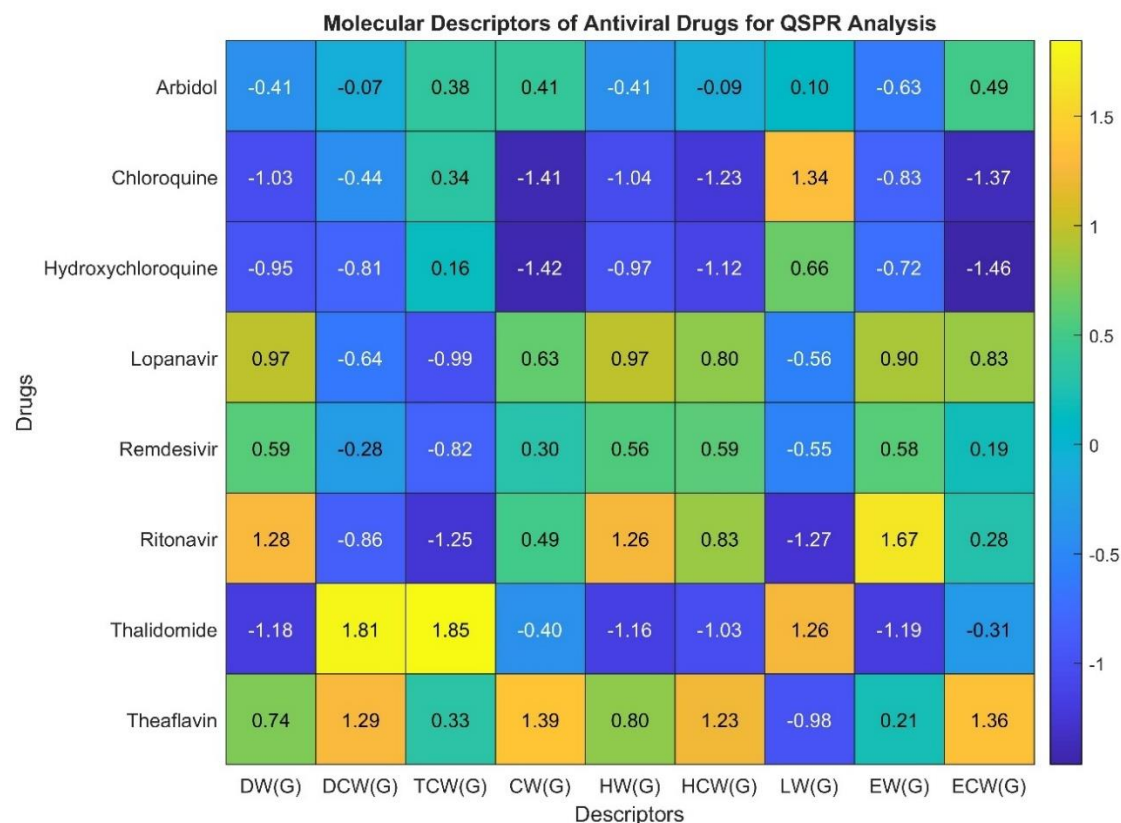
Figure 1: Molecular Descriptors of Antiviral Drugs for QSPR Analysis.
