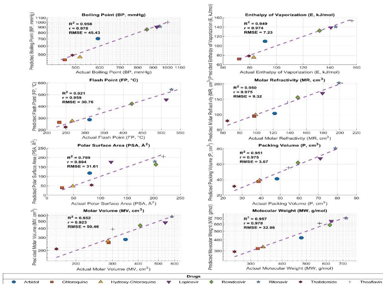
Figure 7. Scatter Plots of Predicted vs. Actual Physicochemical Properties for QSPR Model Validation, Using Marker Shapes with R^2 , r and RMSE.
