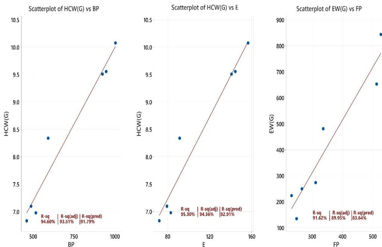
Figure 3: Regression Plots Illustrating Descriptor-Property Relationships Utilized for Remdesivir Data Imputation.
