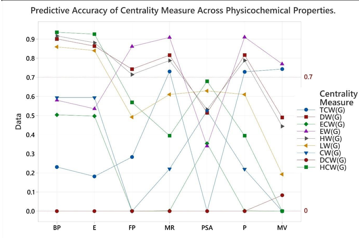
Figure 8. Comparative Predictive Performance ( R^2_{pred} ) of Individual Centrality Measures for Each Physicochemical Property.
