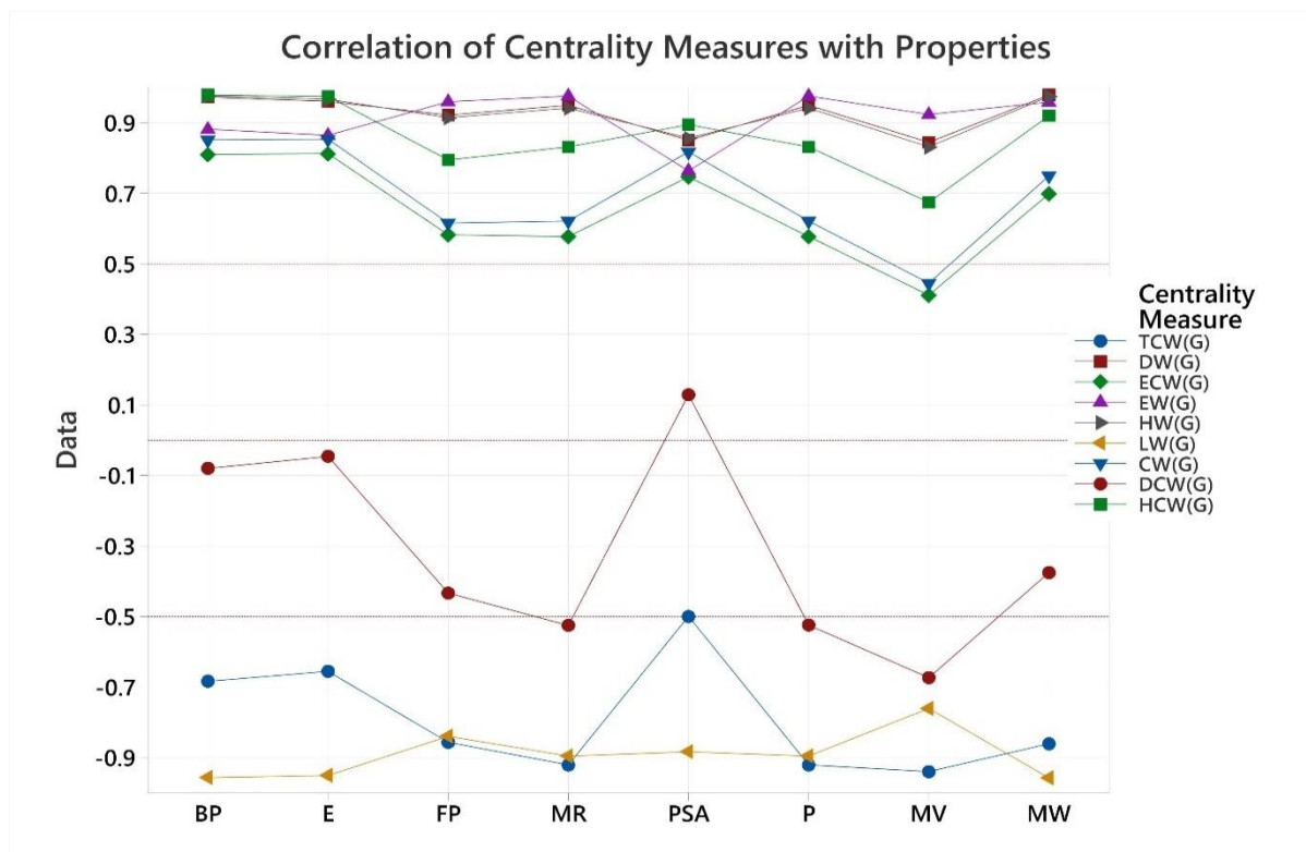
Figure 6: Overall Correlation Trends of Molecular Descriptors Across All Physicochemical Properties.
