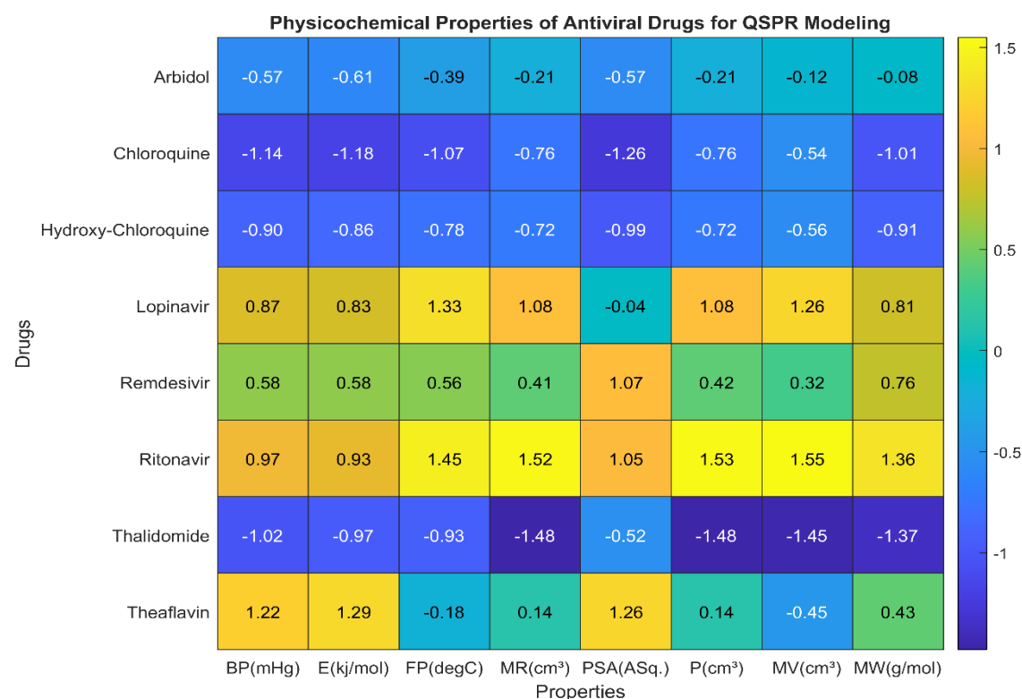
Figure 2: Physicochemical Properties of Antiviral Drugs for QSPR Modelling
