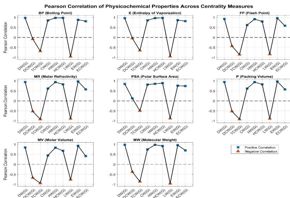
Figure 5: Pearson Correlation Coefficients of Molecular Descriptors with Individual Physicochemical Properties.
