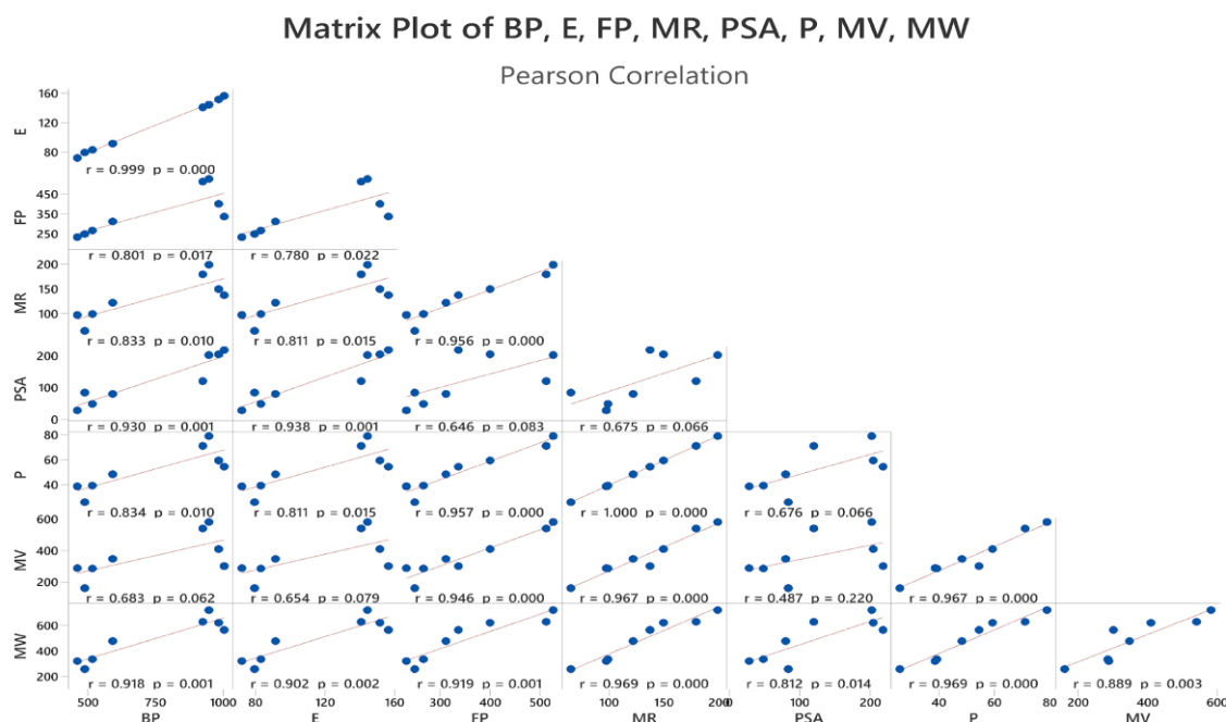
Figure 4: Pearson Correlation Matrix of Physicochemical Properties
