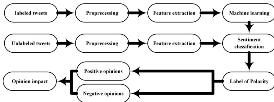
Figure 1. The Operation Flow of Sentiment Analysis of Twitter Data (Giachanou et al.; 2016).
