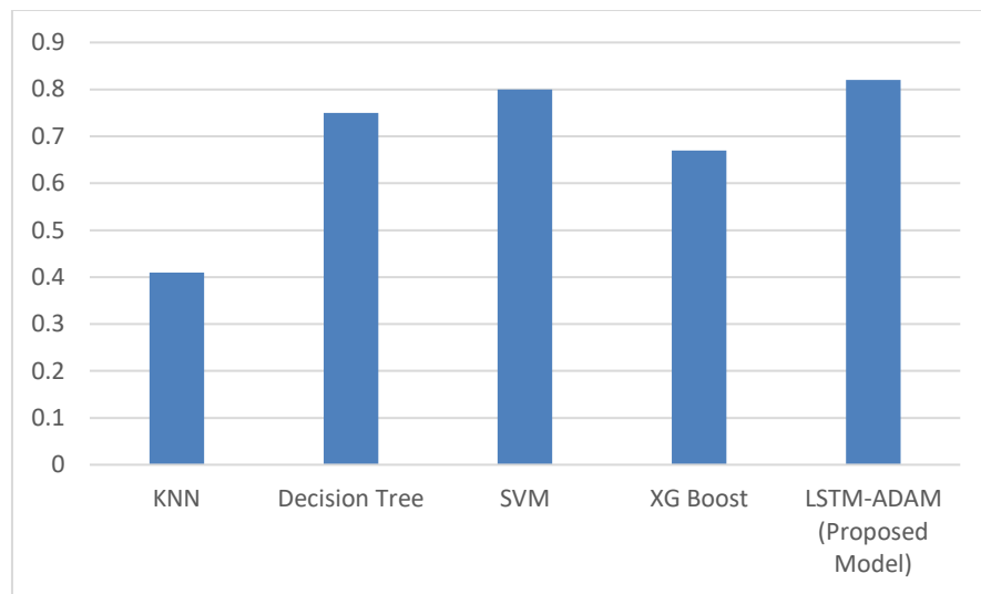
Figure 14. Graphical Analysis of F1-Score among different models and LSTM-ADAM (Proposed Model) for Positive Tweets
