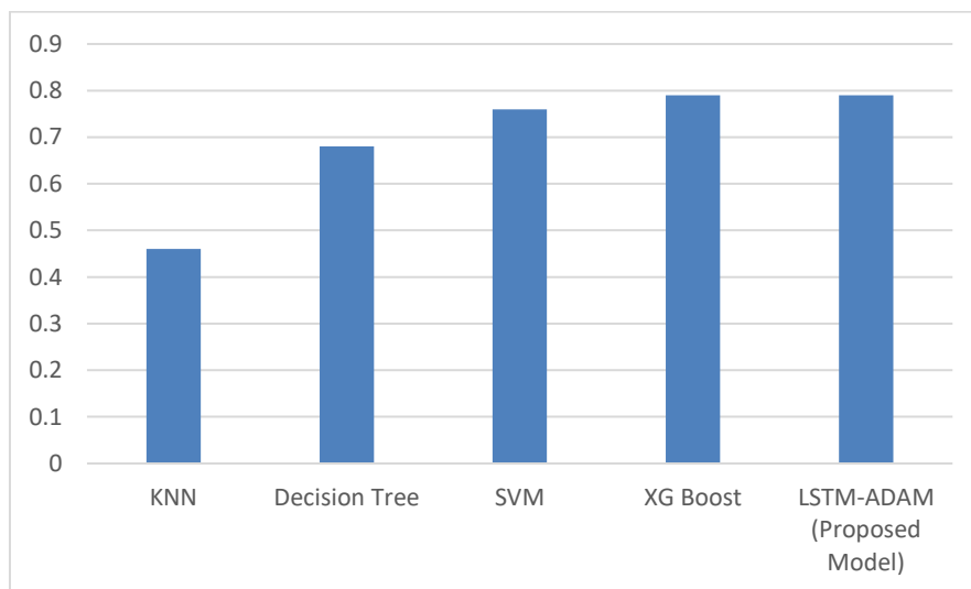
Figure 8. Graphical Analysis of F1-Score among different models and LSTM-ADAM (Proposed Model) for Negative Tweets
