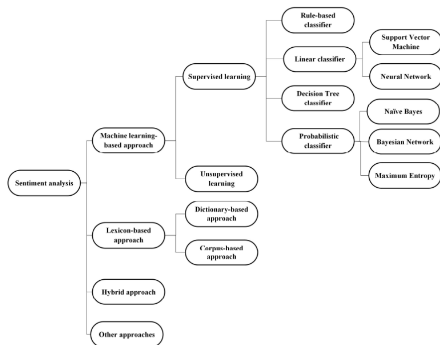
Figure 2. The taxonomy of sentiment analysis (Jose et al.; 2010)
