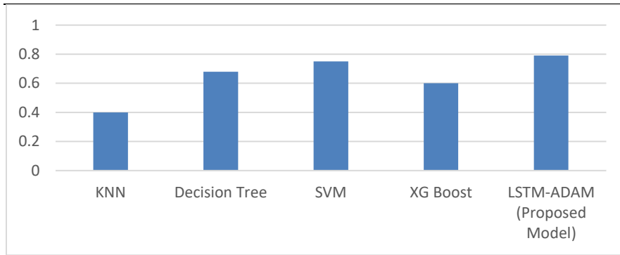
Figure 7. Graphical Analysis of Recall among different models and LSTM-ADAM (Proposed Model) for Negative Tweets
