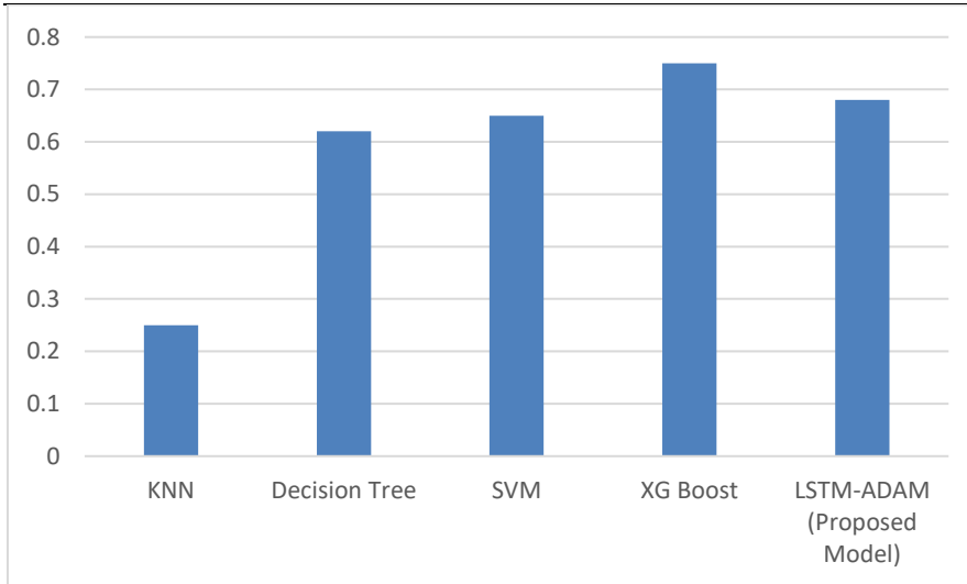
Figure 9. Graphical Analysis of Precision among different models and LSTM-ADAM (Proposed Model) for Neutral Tweets
