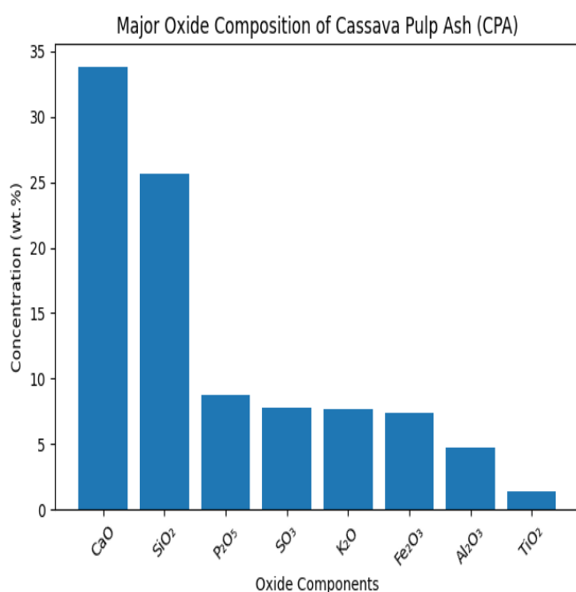
Figure 1: Major oxide composition of CPA
