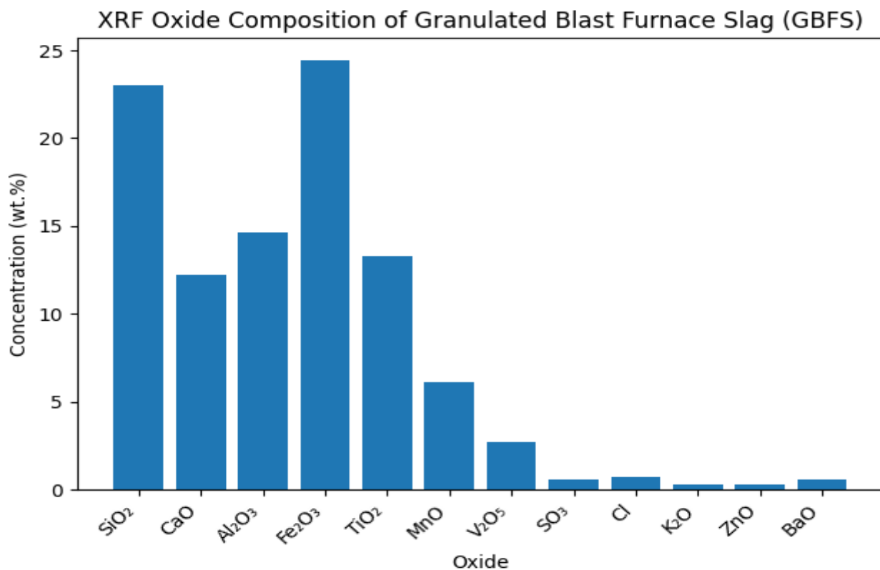
Figure 5: Oxide composition of GBFS
