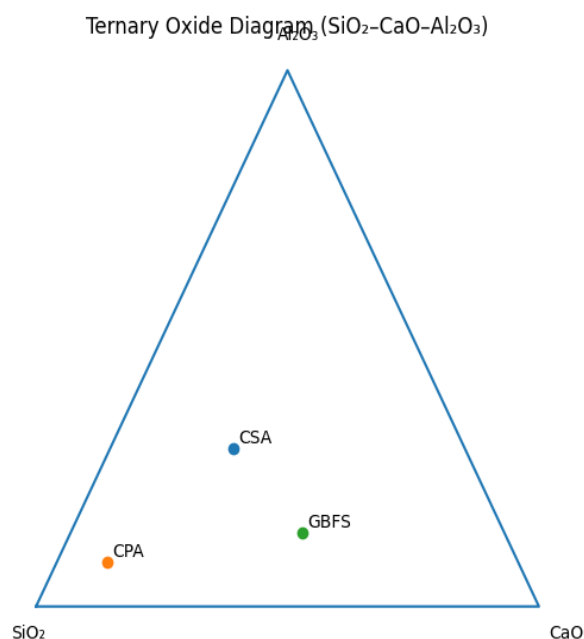
Figure 7: Ternary Oxide Diagram
