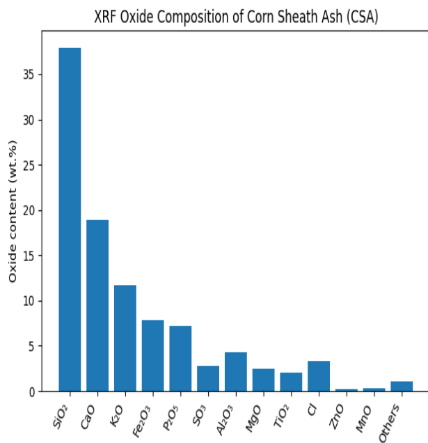
Figure 3: Major oxide composition of CSA
