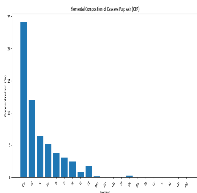
Figure 2: Elemental composition of CPA
