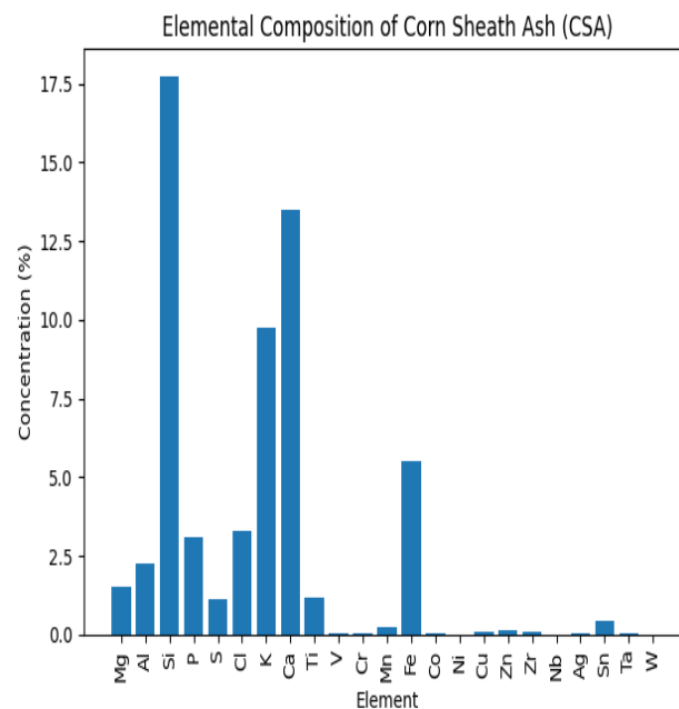
Figure 4: Elemental composition of CSA
