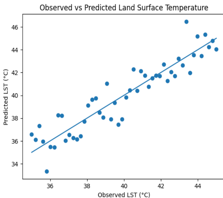
Figure 3. Observed vs. Predicted Land Surface Temperature
