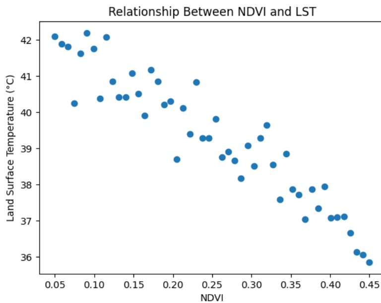
Figure 4. Relationship Between NDVI and Land Surface Temperature
