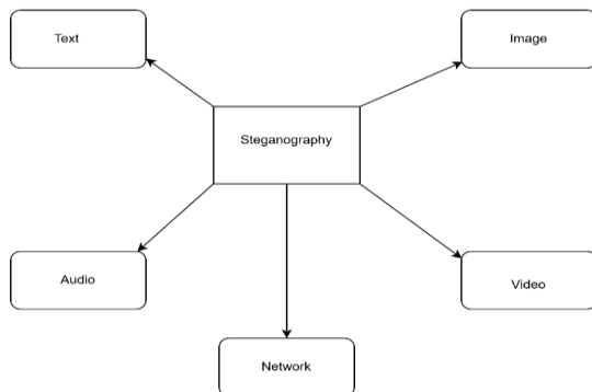
Fig.1 Steganography types
