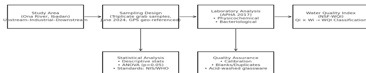
Methodology Workflow for Ona River Water Quality Study
