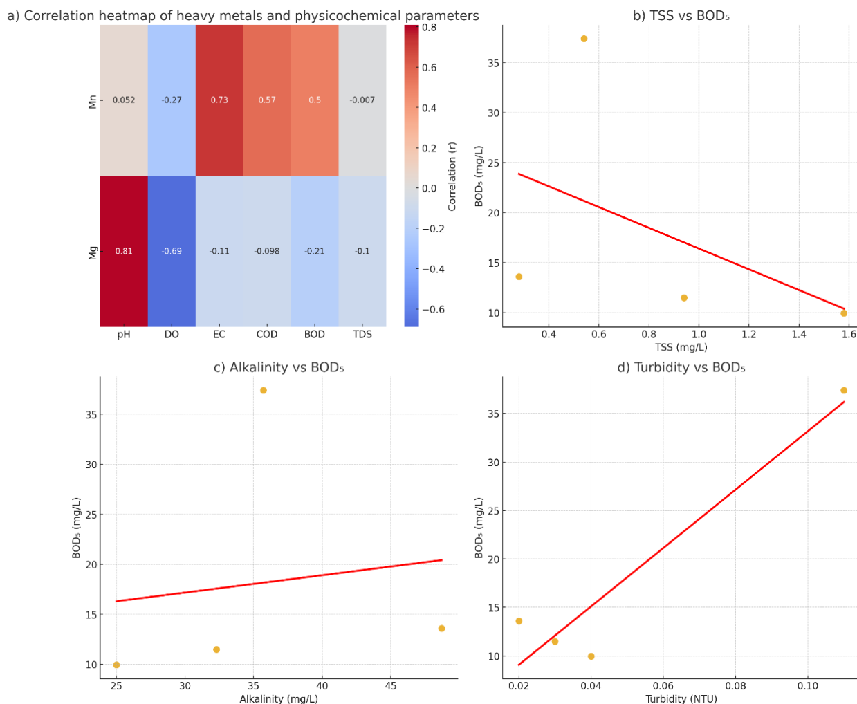
Figure 5a-d. Heatmap visualizes the direction and strength of these correlations, highlighting positive Mn–EC/COD relationships and negative Mg–DO association.
