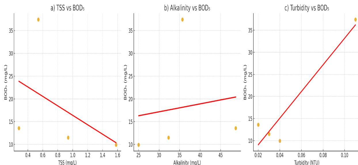
Figure 6a-c. Nutrients vs BOD 5 : a) TSS vs BOD 5 ; b) Alkalinity vs BOD 5 ; c) Turbidity vs BOD 5
