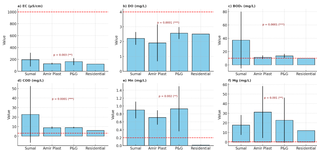
Figure 3. Multi-panel illustration of physicochemical parameters of Ona River across industrial and residential sites: a) Electrical conductivity (EC), b) Dissolved oxygen (DO), c) Biochemical oxygen demand (BOD 5 ), d) Chemical oxygen demand (COD), e) Manganese (Mn), and f) Magnesium (Mg). Bars represent mean \pm standard deviation (SD).
