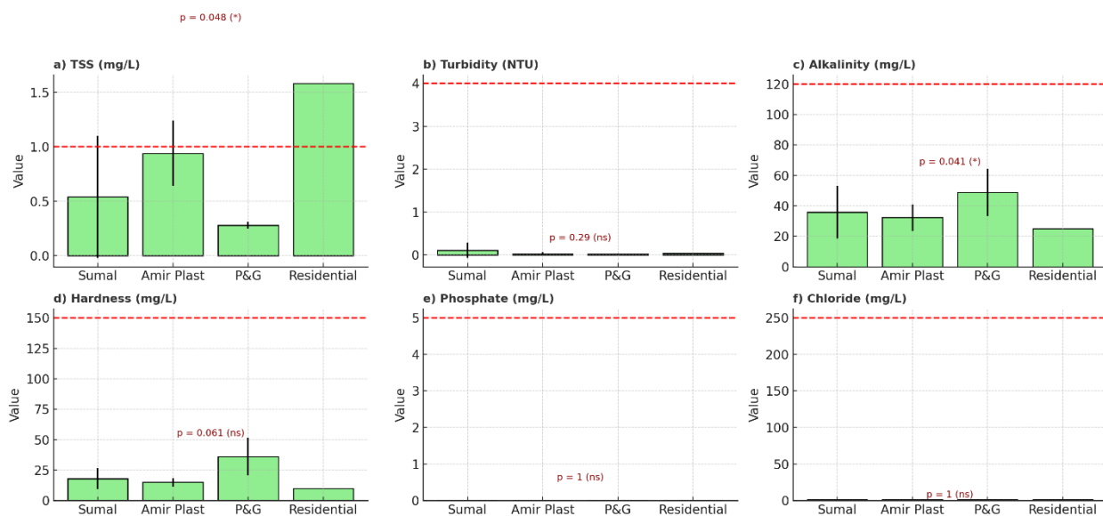
Figure 4. Multi-panel illustration of nutrients and major ions in Ona River:
