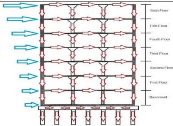
Figure 1. Global seismic load path in a multi-storey building.
