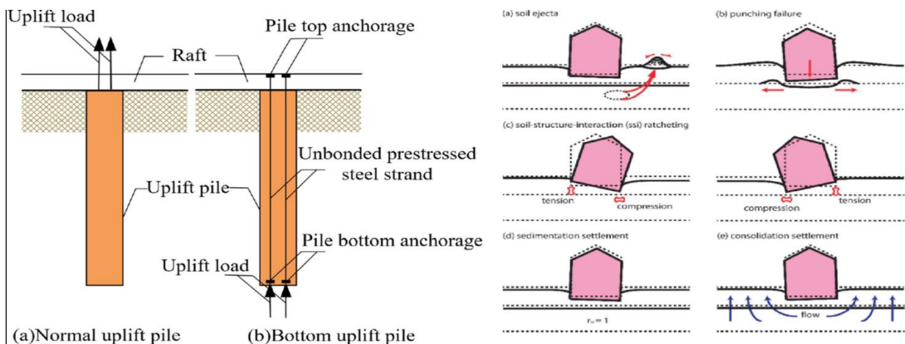
Fig. 5. Insight: Overturning vs Bearing
