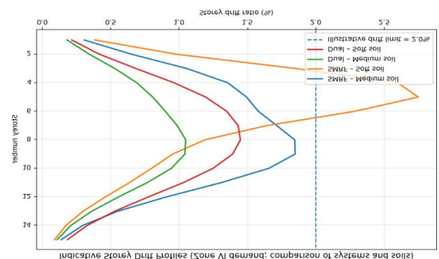
Graph 2: Indicative Storey Drift Profiles (Zone VI demand; comparison of system and soil
