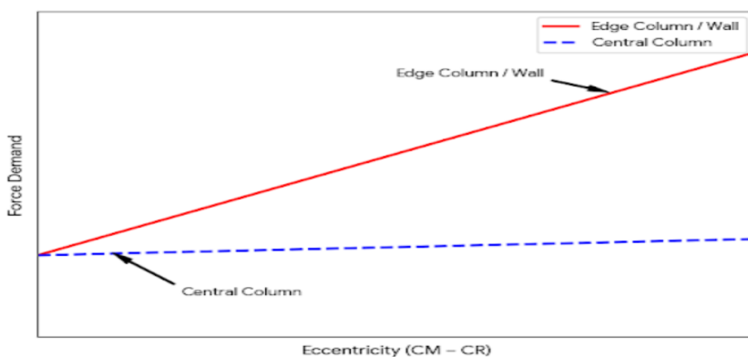
Graph 5: Torsional amplification of edge elements
