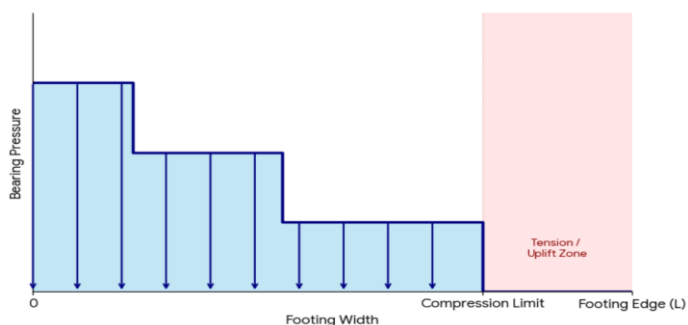
Graph 7: Bearing pressure distribution under seismic overturning
