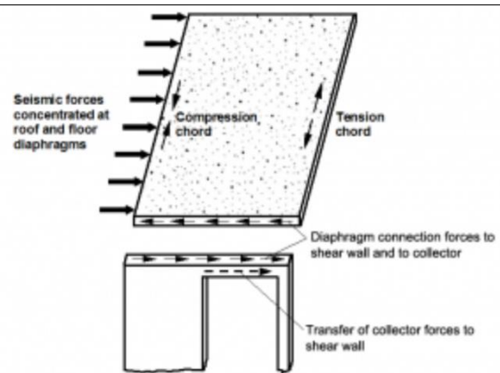
Figure 2. Diaphragm action and collector force transfer mechanism.
