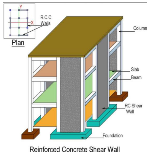
Fig. 4: Shear Walls or Braced Frames
