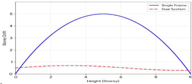
Graph 4: Storey drift comparison – single frame vs dual system
