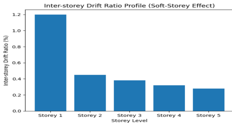
Graph 6: Inter-storey drift ratio profile (soft-storey effect) (Shown as a bar chart with a 1.20% drift spike at the first storey.)
