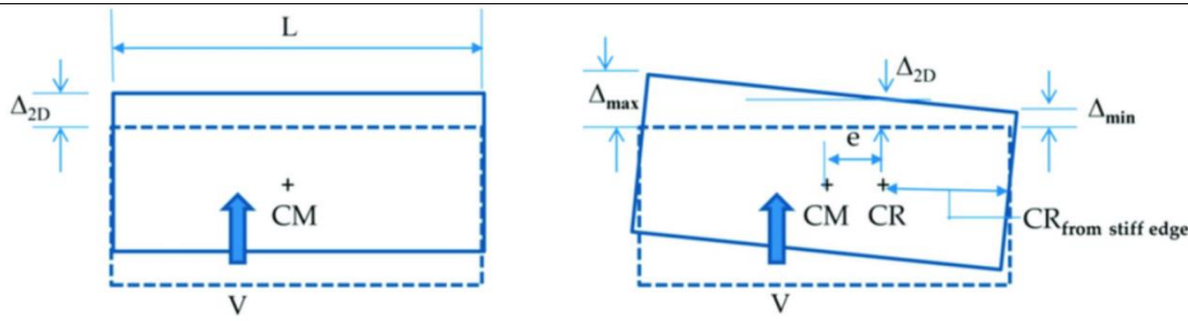
(a) A 3D analysis model restrained from rotation about the vertical axis
