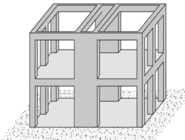
Fig.3 : Moment Resisting Frames (MRF)
