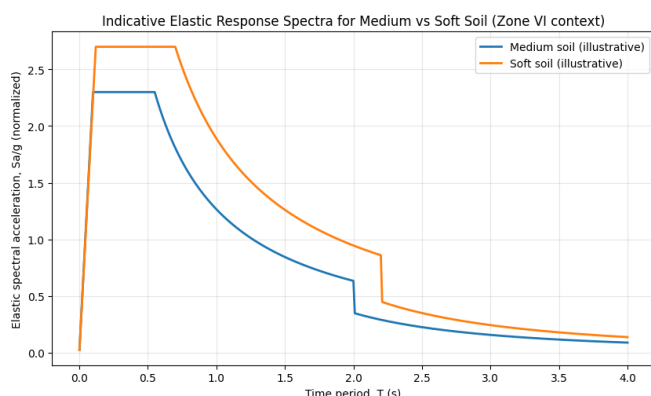
Graph 1 : Indicative Elastic Response Spectra for Medium vs Soft Soil
