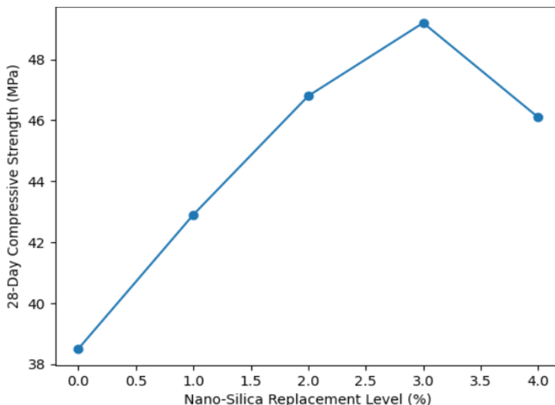
Effect of Nano-Silica Content on 28-Day Compressive Strength
