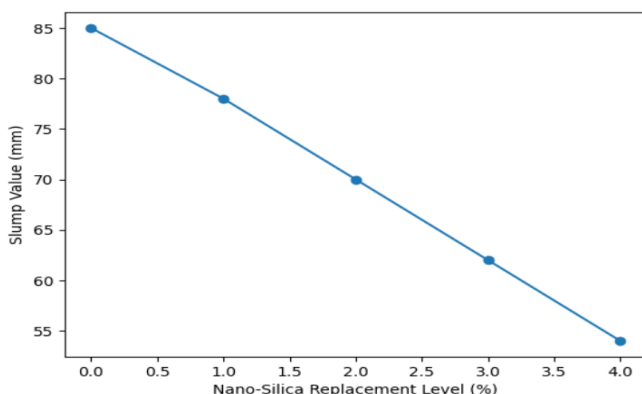
Variation of Concrete Workability with Nano-Silica Content
