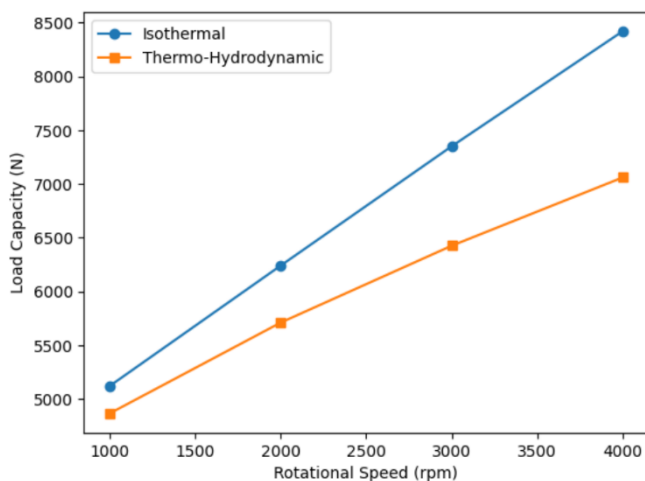
Fig. 1. Influence of Rotational Speed on Journal Bearing Load Support under Thermal Effects
