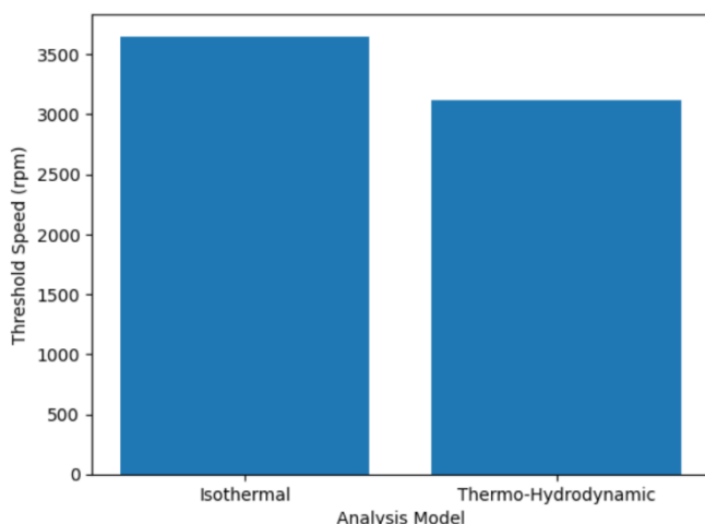
Fig. 3. Effect of Thermal Modeling on the Stability Limit of Journal Bearings
