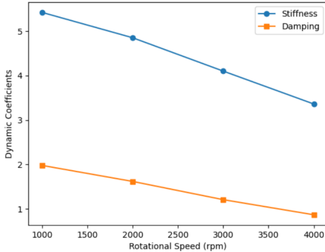
Fig. 2. Variation of Bearing Stiffness and Damping with Increasing Operating Speed
