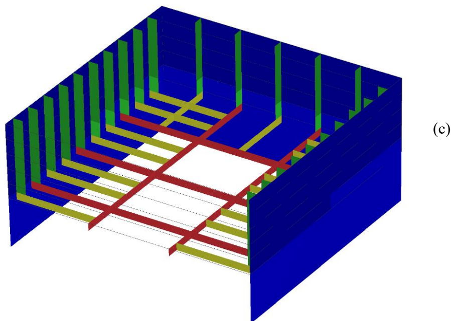
Figure 4: Three types of excavation design: (a) One rib walls before every cross wall in both directions (b) Two rib walls before every cross wall in both directions (c) Two rib walls before every cross wall in long direction and One rib wall before every cross wall in short direction
