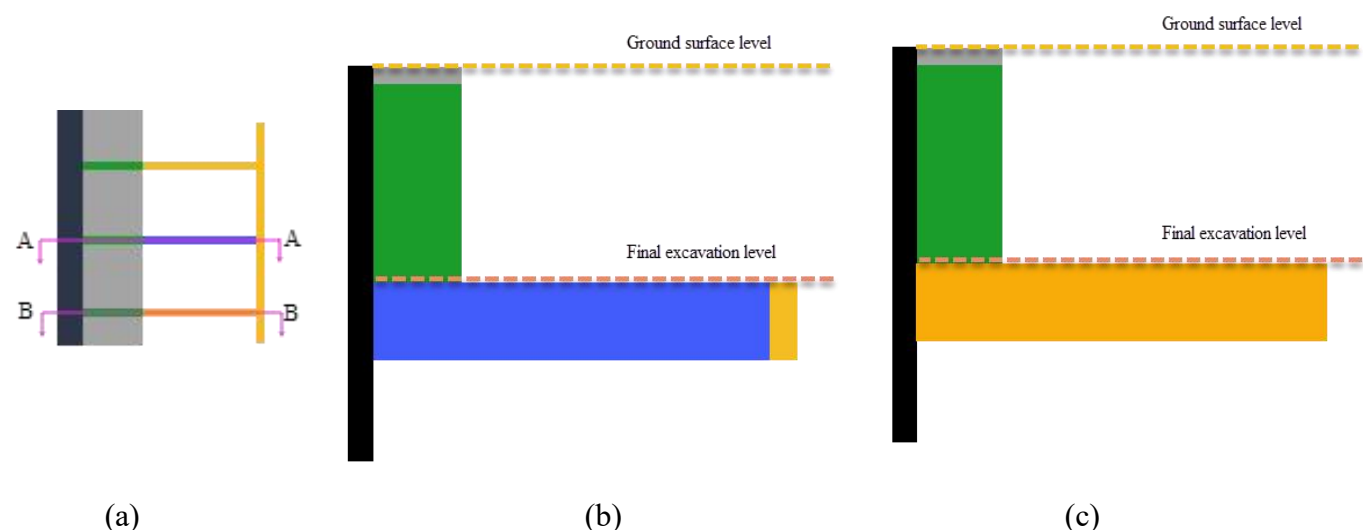
Figure 3: The schematic diagram of the RFD system wall: a) part of plan view, b) cross section A-A, c) cross section B-B
