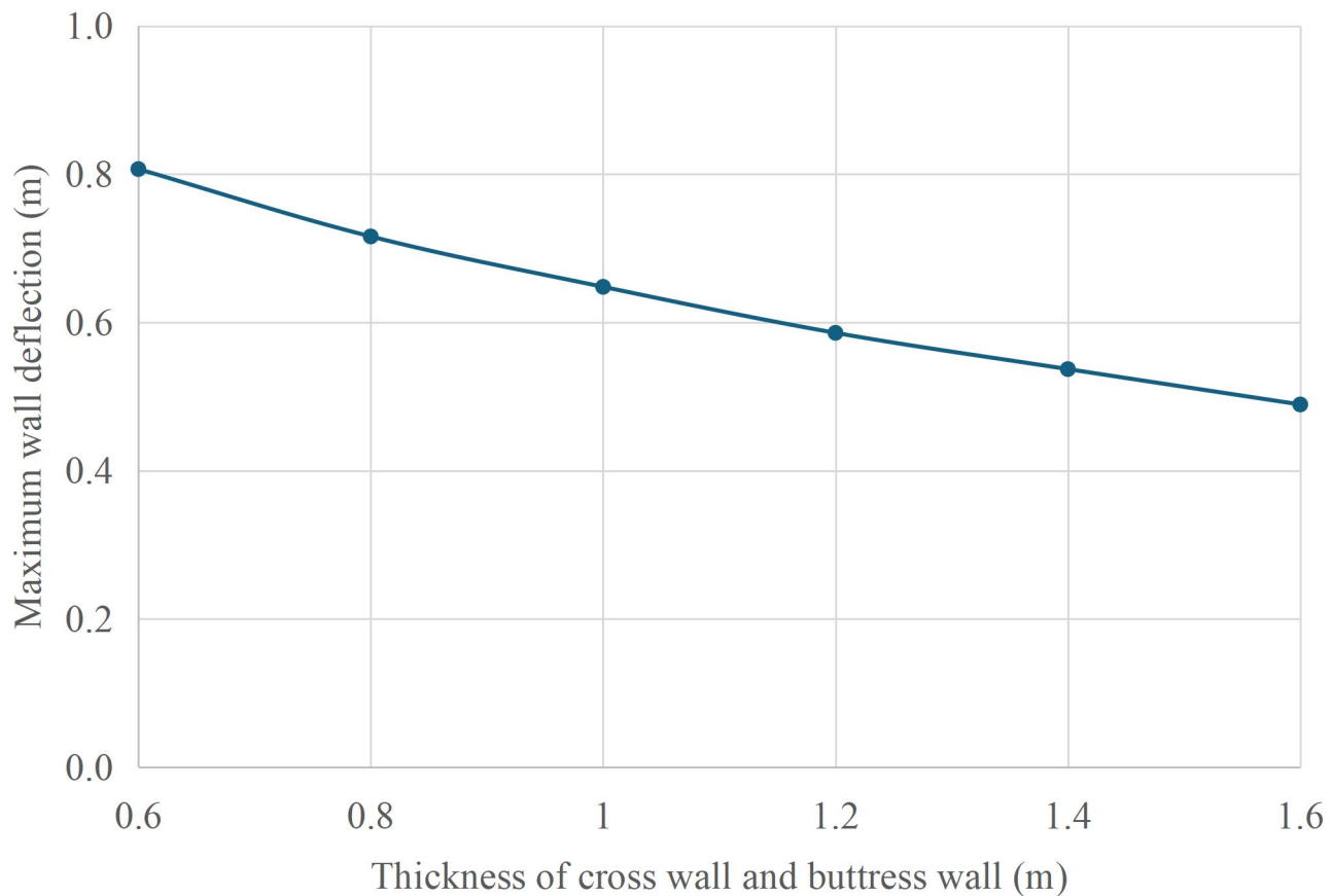
Figure 8: The maximum wall deflection on different thickness of cross wall and buttress wall all and buttress wall (a) long direction (b) short direction
