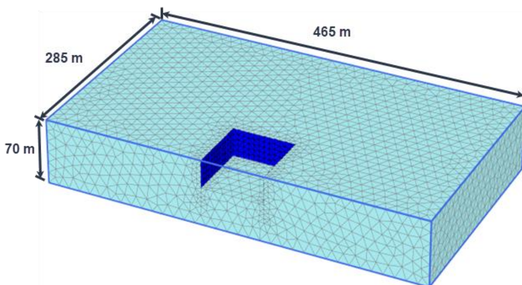
Figure 1: Typical geometry and finite element mesh used for analysis
