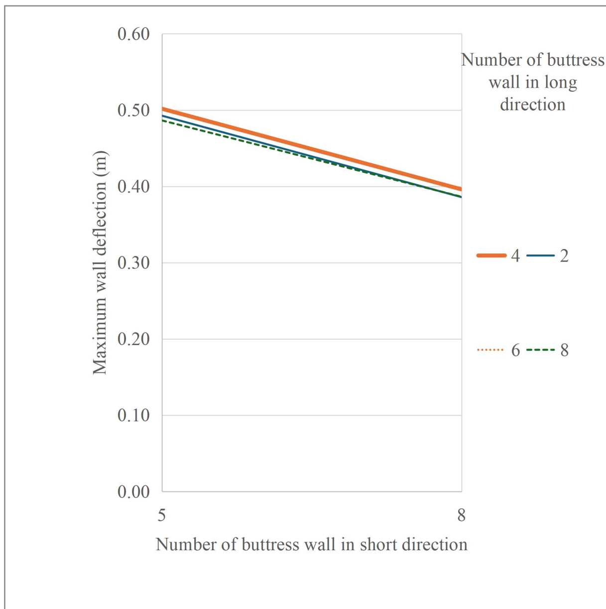
Figure 7: The maximum wall deflection in a short direction for different number of cross walls in both directions (type 2)
