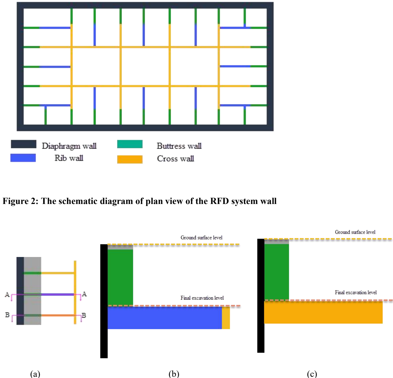
Figure 3: The schematic diagram of the RFD system wall: a) part of plan view, b) cross section A-A, c) cross section B-B
